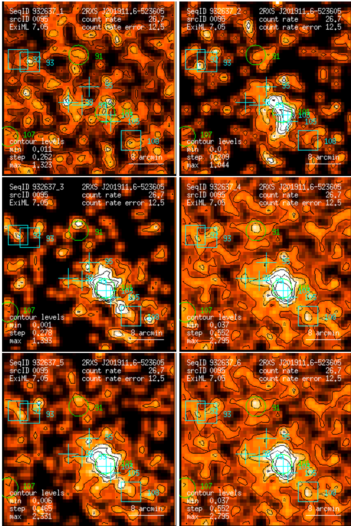
Figure 95: RASS 932637: detection 0095: band rate images, Gaussian filter: (1) PSPC channels 11 – 41, (2) 52 – 90, (3) 91 – 201, (4) 11 – 235, (5) 52 – 201, (6) 11 – 201. Broad band rates in counts/ks. Band rate contour levels in counts/ks/arcmin 2 .
