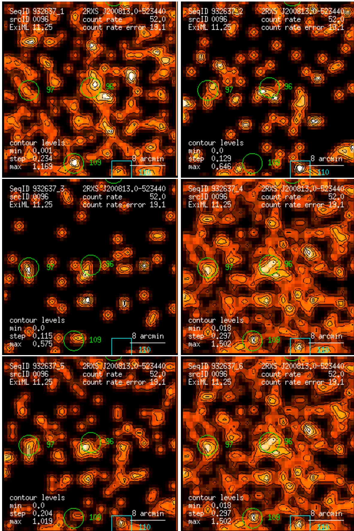
Figure 96: RASS 932637: detection 0096: band rate images, Gaussian filter: (1) PSPC channels 11 – 41, (2) 52 – 90, (3) 91 – 201, (4) 11 – 235, (5) 52 – 201, (6) 11 – 201. Broad band rates in counts/ks. Band rate contour levels in counts/ks/arcmin 2 .
