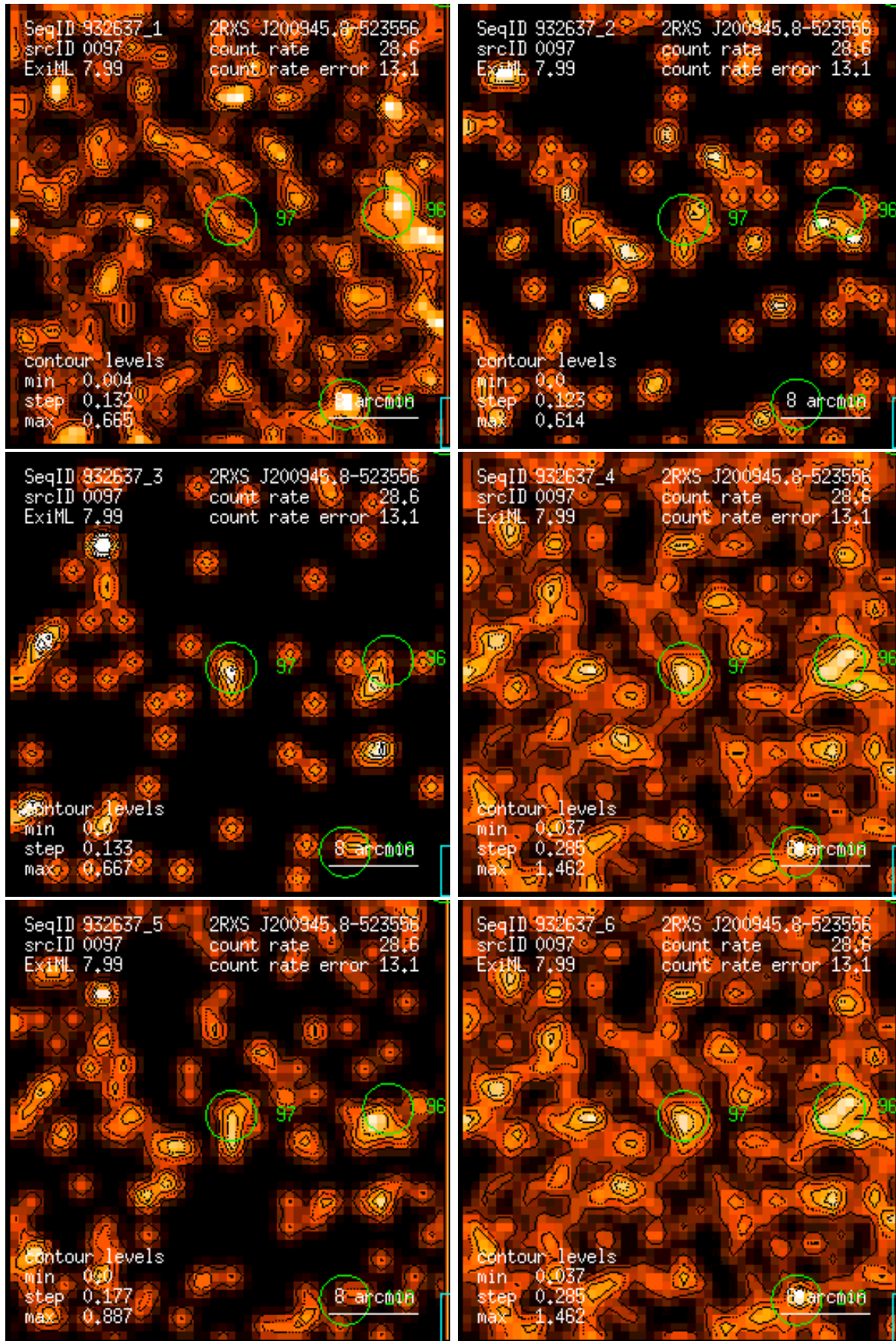
Figure 97: RASS 932637: detection 0097: band rate images, Gaussian filter: (1) PSPC channels 11 – 41, (2) 52 – 90, (3) 91 – 201, (4) 11 – 235, (5) 52 – 201, (6) 11 – 201. Broad band rates in counts/ks. Band rate contour levels in counts/ks/arcmin 2 .
