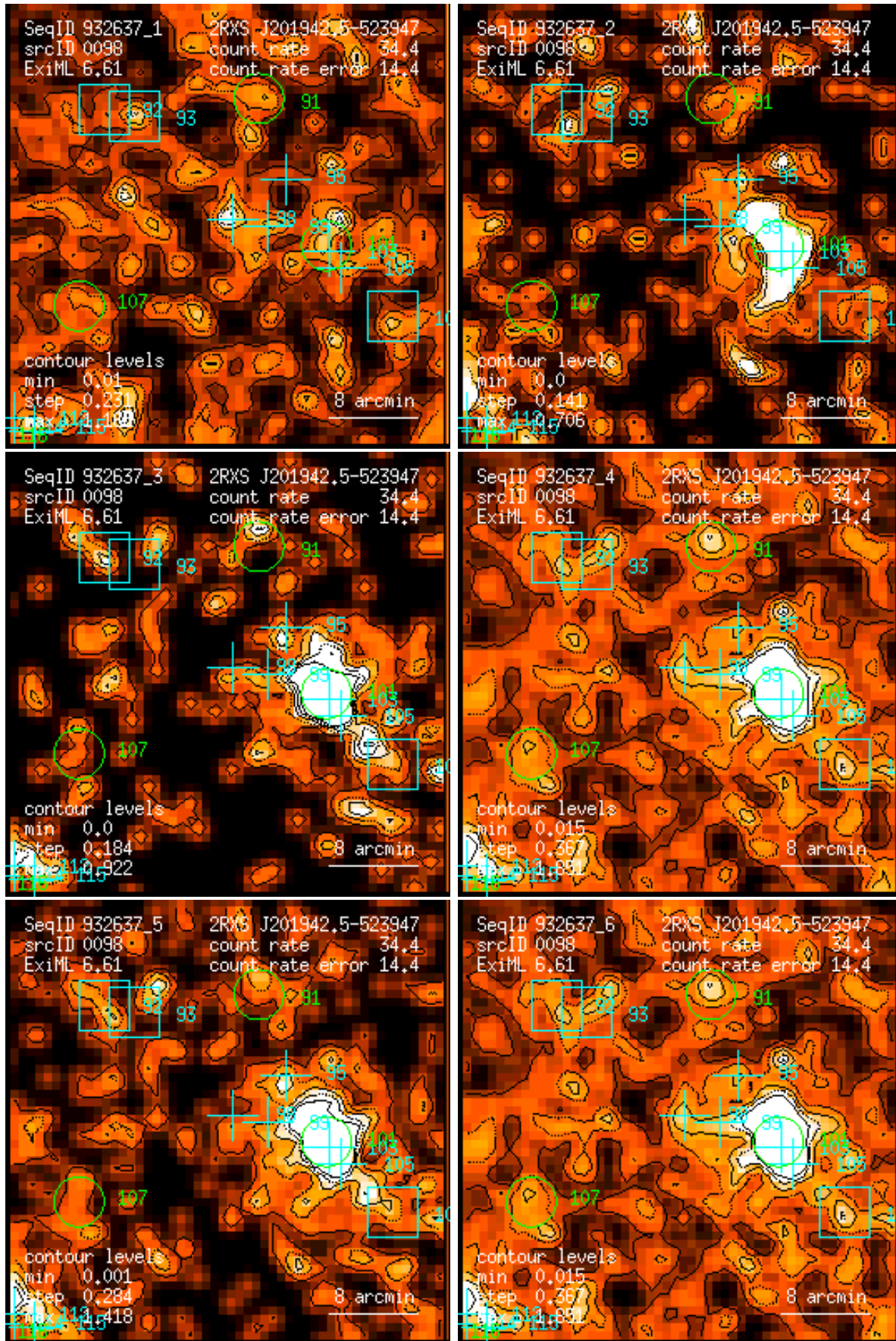
Figure 98: RASS 932637: detection 0098: band rate images, Gaussian filter: (1) PSPC channels 11 – 41, (2) 52 – 90, (3) 91 – 201, (4) 11 – 235, (5) 52 – 201, (6) 11 – 201. Broad band rates in counts/ks. Band rate contour levels in counts/ks/arcmin 2 .
