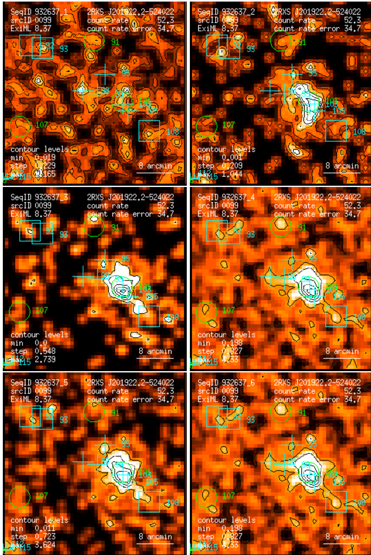
Figure 99: RASS 932637: detection 0099: band rate images, Gaussian filter: (1) PSPC channels 11 – 41, (2) 52 – 90, (3) 91 – 201, (4) 11 – 235, (5) 52 – 201, (6) 11 – 201. Broad band rates in counts/ks. Band rate contour levels in counts/ks/arcmin 2 .
