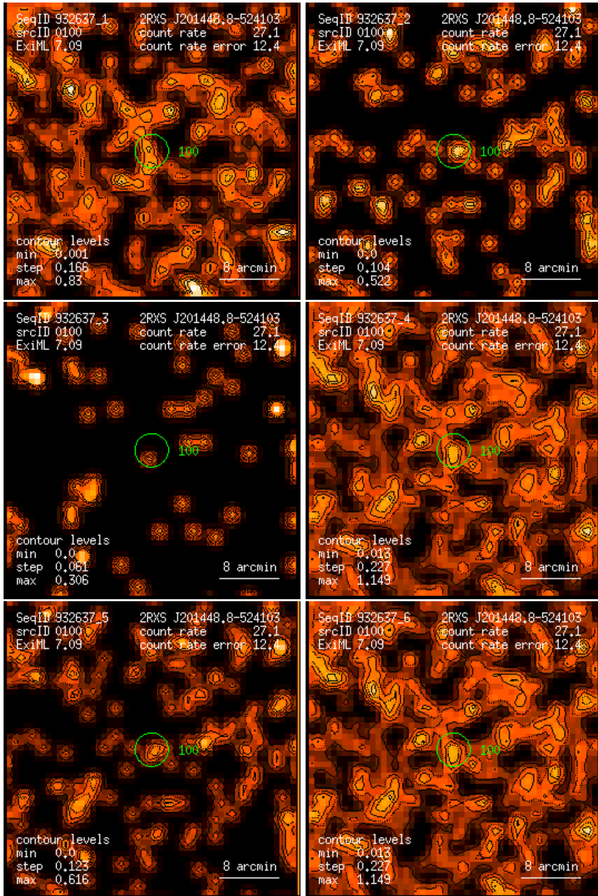
Figure 100: RASS 932637: detection 0100: band rate images, Gaussian filter: (1) PSPC channels 11 – 41, (2) 52 – 90, (3) 91 – 201, (4) 11 – 235, (5) 52 – 201, (6) 11 – 201. Broad band rates in counts/ks. Band rate contour levels in counts/ks/arcmin 2 .
