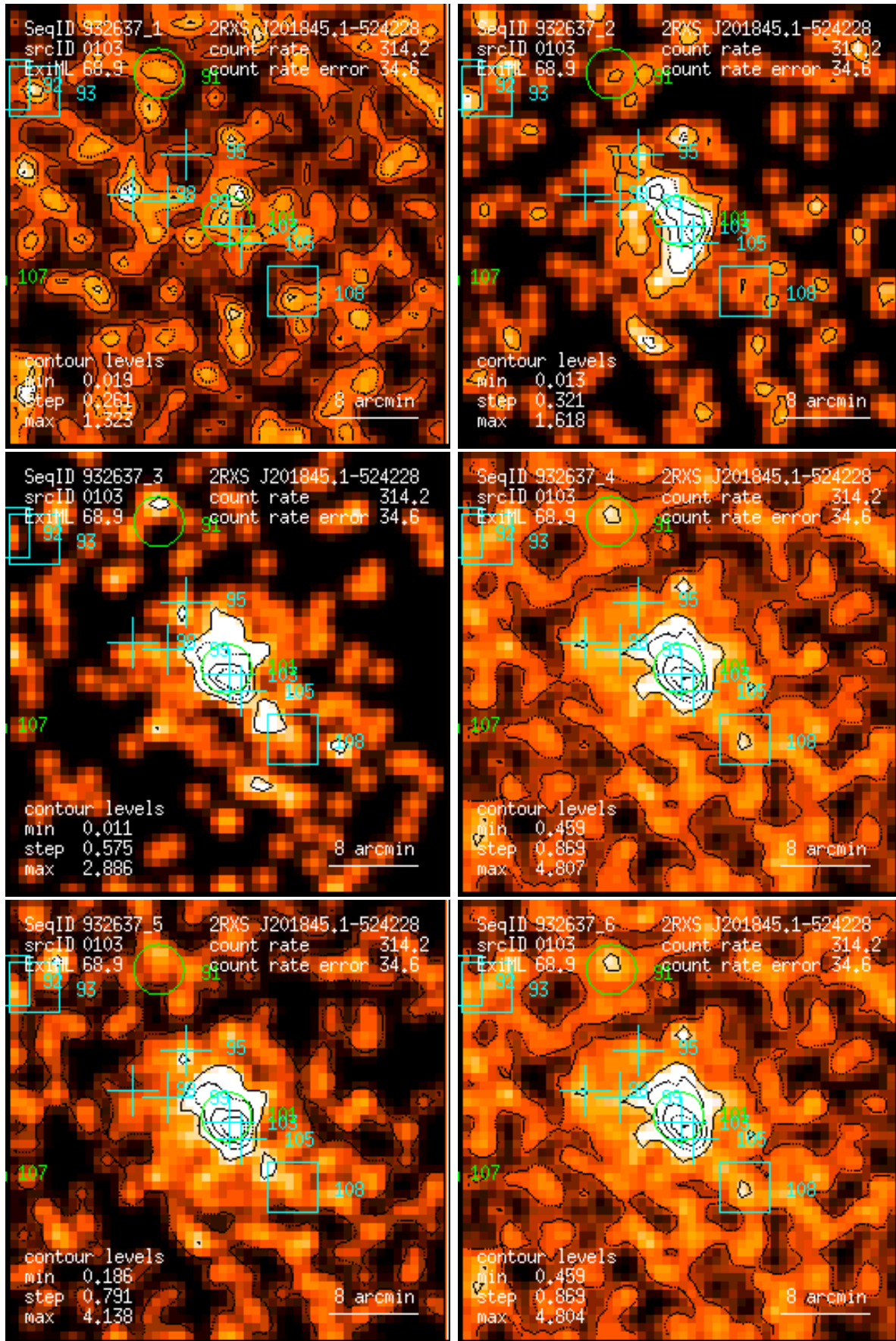
Figure 103: RASS 932637: detection 0103: band rate images, Gaussian filter: (1) PSPC channels 11 – 41, (2) 52 – 90, (3) 91 – 201, (4) 11 – 235, (5) 52 – 201, (6) 11 – 201. Broad band rates in counts/ks. Band rate contour levels in counts/ks/arcmin 2 .
