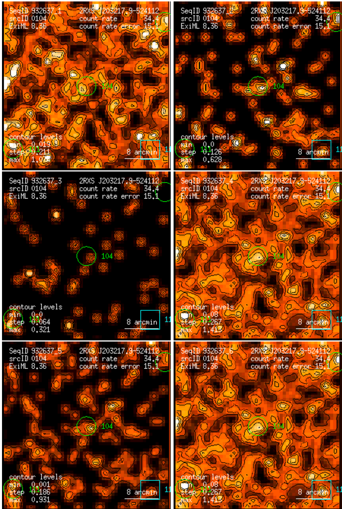
Figure 104: RASS 932637: detection 0104: band rate images, Gaussian filter: (1) PSPC channels 11 – 41, (2) 52 – 90, (3) 91 – 201, (4) 11 – 235, (5) 52 – 201, (6) 11 – 201. Broad band rates in counts/ks. Band rate contour levels in counts/ks/arcmin 2 .
