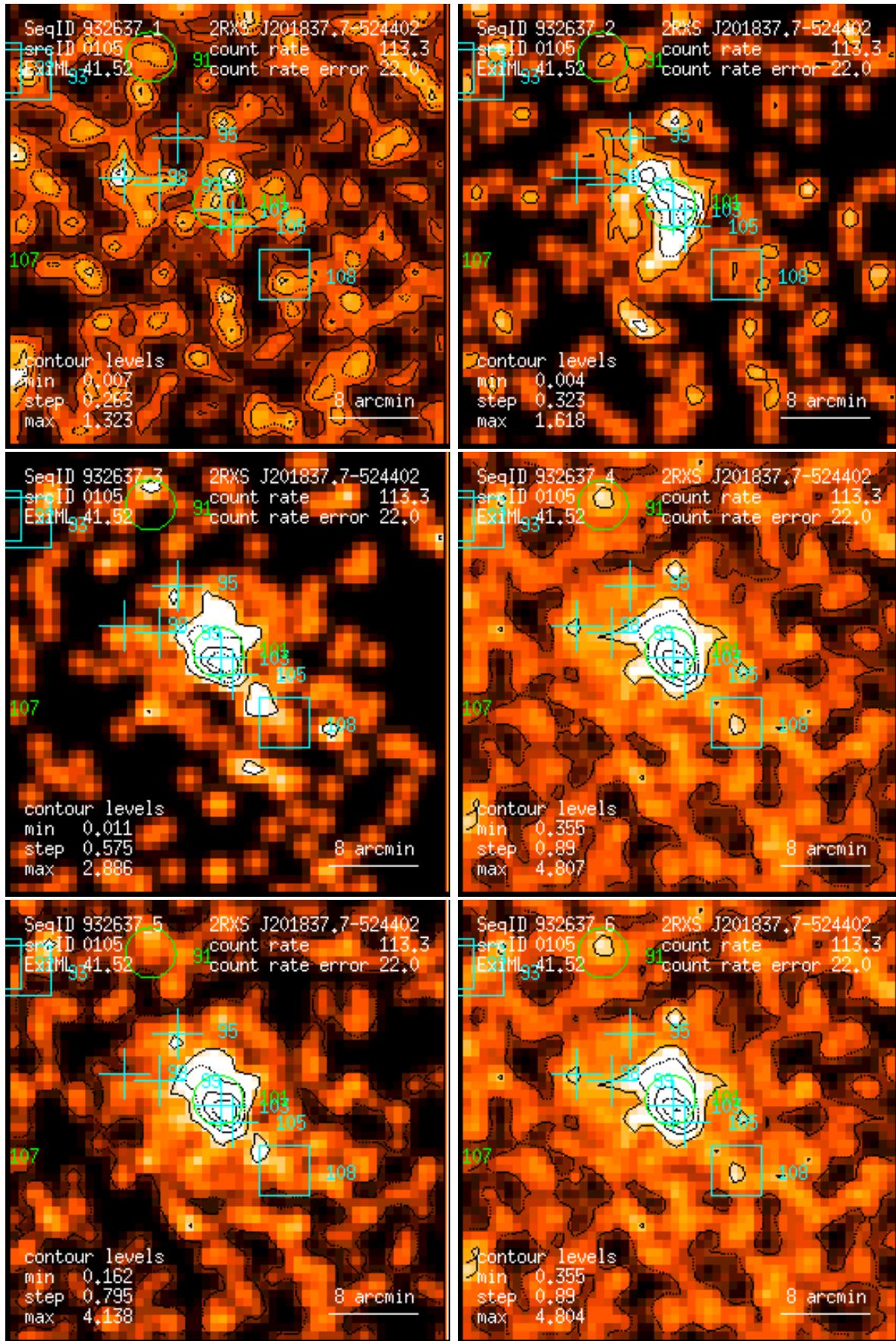
Figure 105: RASS 932637: detection 0105: band rate images, Gaussian filter: (1) PSPC channels 11 – 41, (2) 52 – 90, (3) 91 – 201, (4) 11 – 235, (5) 52 – 201, (6) 11 – 201. Broad band rates in counts/ks. Band rate contour levels in counts/ks/arcmin 2 .
