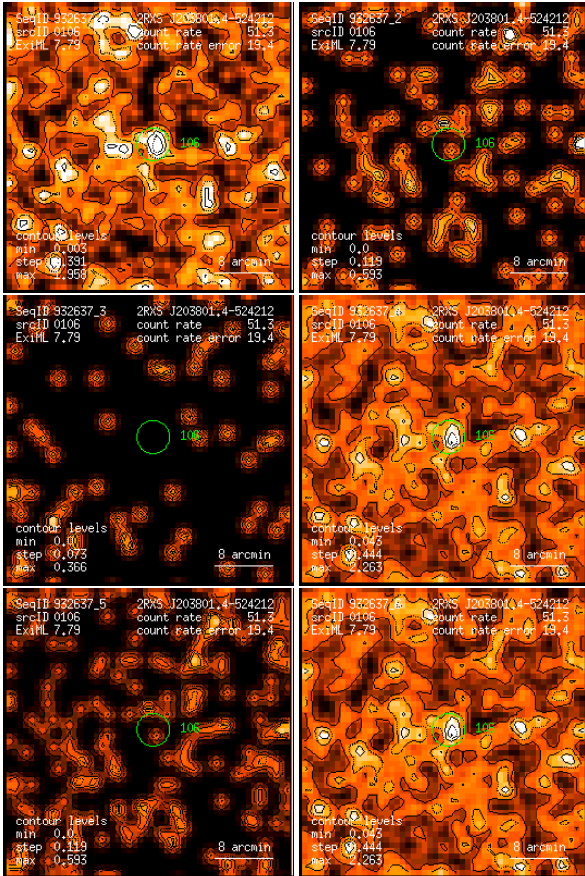
Figure 106: RASS 932637: detection 0106: band rate images, Gaussian filter: (1) PSPC channels 11 – 41, (2) 52 – 90, (3) 91 – 201, (4) 11 – 235, (5) 52 – 201, (6) 11 – 201. Broad band rates in counts/ks. Band rate contour levels in counts/ks/arcmin 2 .
