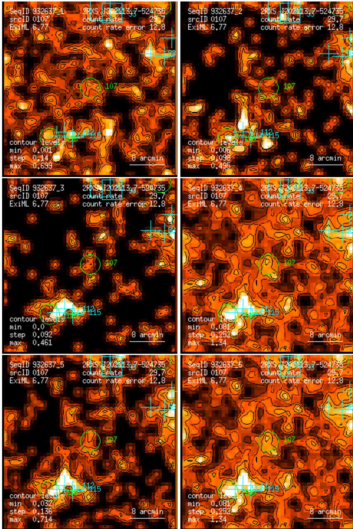
Figure 107: RASS 932637: detection 0107: band rate images, Gaussian filter: (1) PSPC channels 11 – 41, (2) 52 – 90, (3) 91 – 201, (4) 11 – 235, (5) 52 – 201, (6) 11 – 201. Broad band rates in counts/ks. Band rate contour levels in counts/ks/arcmin 2 .
