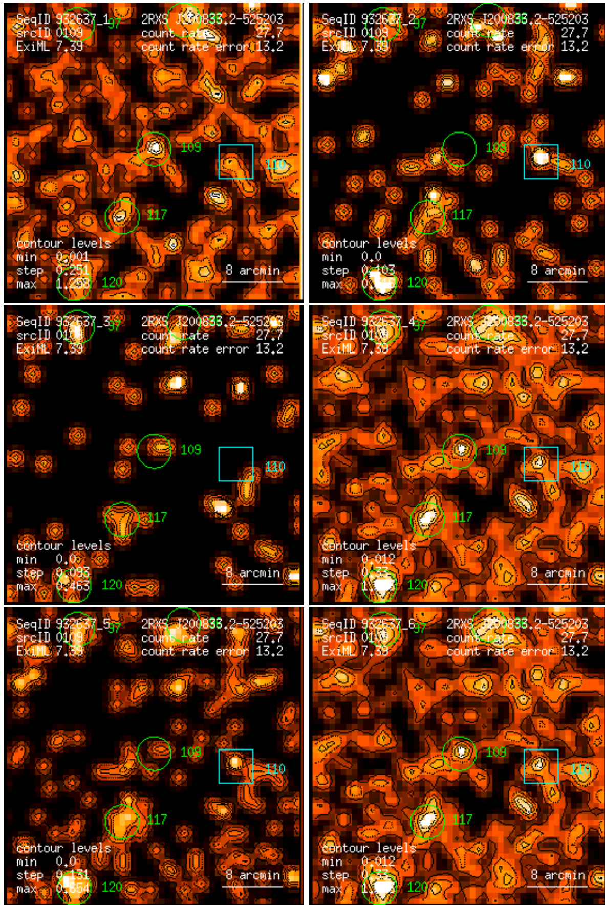
Figure 109: RASS 932637: detection 0109: band rate images, Gaussian filter: (1) PSPC channels 11 – 41, (2) 52 – 90, (3) 91 – 201, (4) 11 – 235, (5) 52 – 201, (6) 11 – 201. Broad band rates in counts/ks. Band rate contour levels in counts/ks/arcmin 2 .
