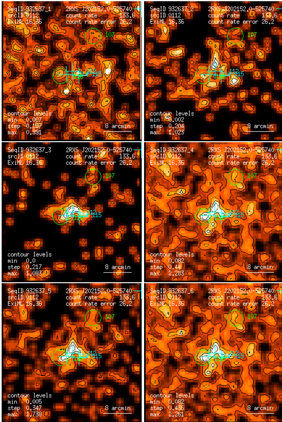
Figure 112: RASS 932637: detection 0112: band rate images, Gaussian filter: (1) PSPC channels 11 – 41, (2) 52 – 90, (3) 91 – 201, (4) 11 – 235, (5) 52 – 201, (6) 11 – 201. Broad band rates in counts/ks. Band rate contour levels in counts/ks/arcmin 2 .
