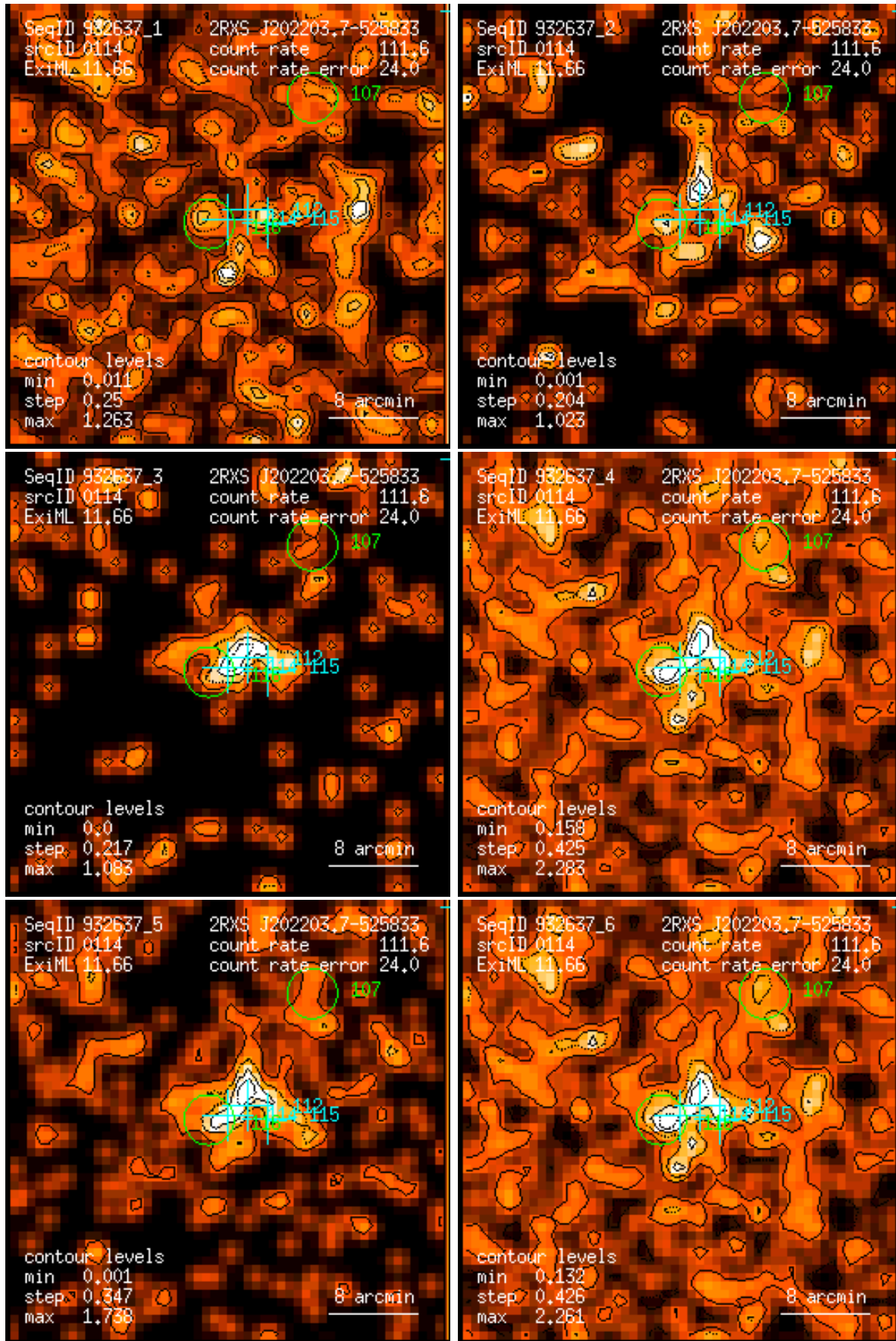
Figure 114: RASS 932637: detection 0114: band rate images, Gaussian filter: (1) PSPC channels 11 – 41, (2) 52 – 90, (3) 91 – 201, (4) 11 – 235, (5) 52 – 201, (6) 11 – 201. Broad band rates in counts/ks. Band rate contour levels in counts/ks/arcmin 2 .
