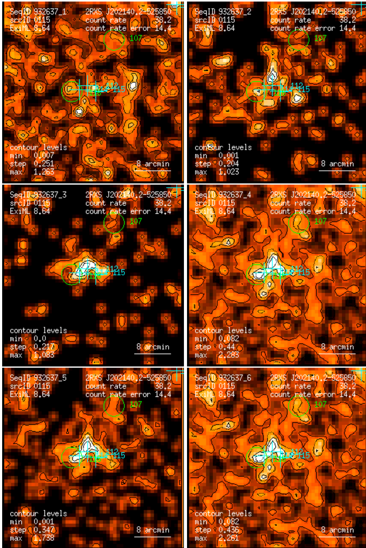
Figure 115: RASS 932637: detection 0115: band rate images, Gaussian filter: (1) PSPC channels 11 – 41, (2) 52 – 90, (3) 91 – 201, (4) 11 – 235, (5) 52 – 201, (6) 11 – 201. Broad band rates in counts/ks. Band rate contour levels in counts/ks/arcmin 2 .
