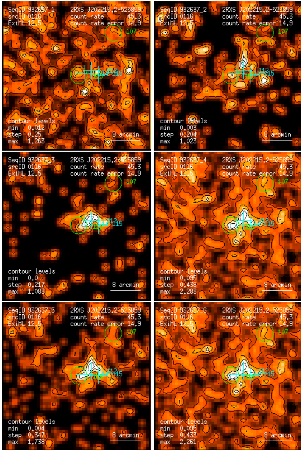
Figure 116: RASS 932637: detection 0116: band rate images, Gaussian filter: (1) PSPC channels 11 – 41, (2) 52 – 90, (3) 91 – 201, (4) 11 – 235, (5) 52 – 201, (6) 11 – 201. Broad band rates in counts/ks. Band rate contour levels in counts/ks/arcmin 2 .
