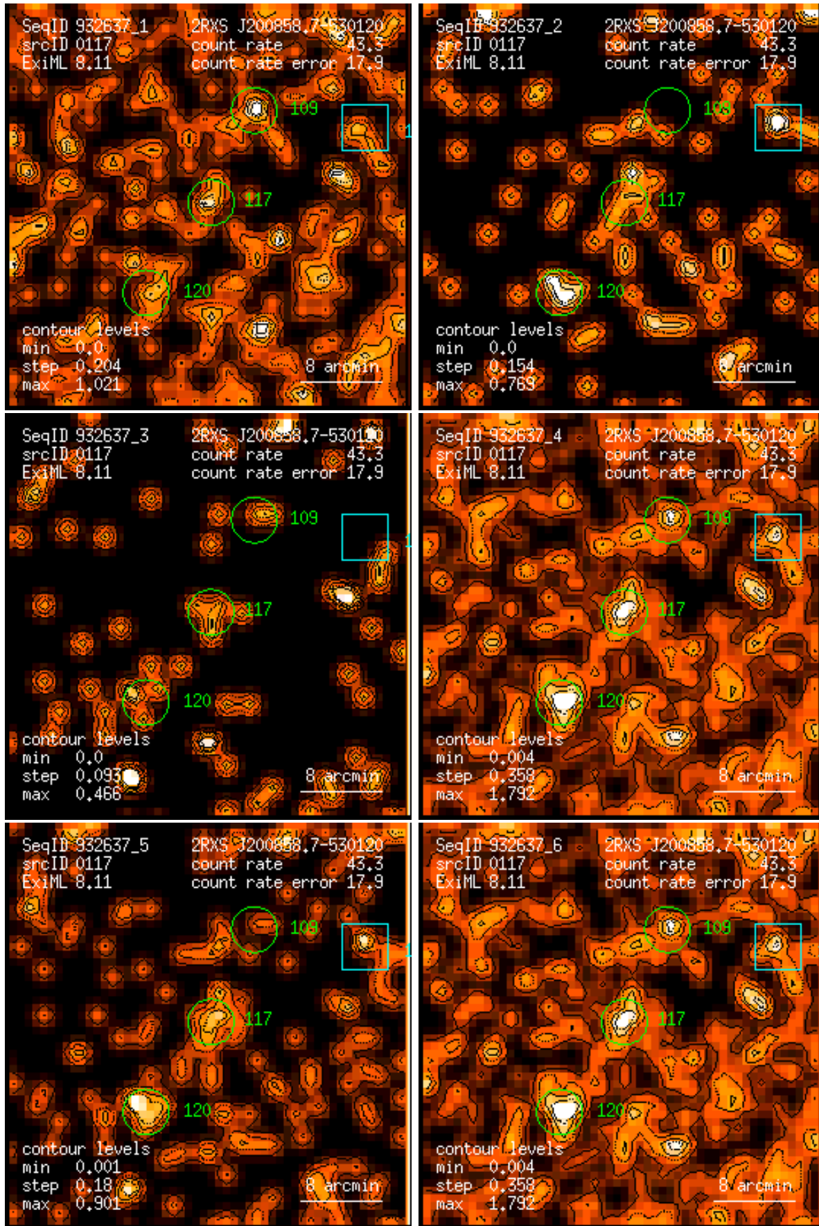
Figure 117: RASS 932637: detection 0117: band rate images, Gaussian filter: (1) PSPC channels 11 – 41, (2) 52 – 90, (3) 91 – 201, (4) 11 – 235, (5) 52 – 201, (6) 11 – 201. Broad band rates in counts/ks. Band rate contour levels in counts/ks/arcmin 2 .
