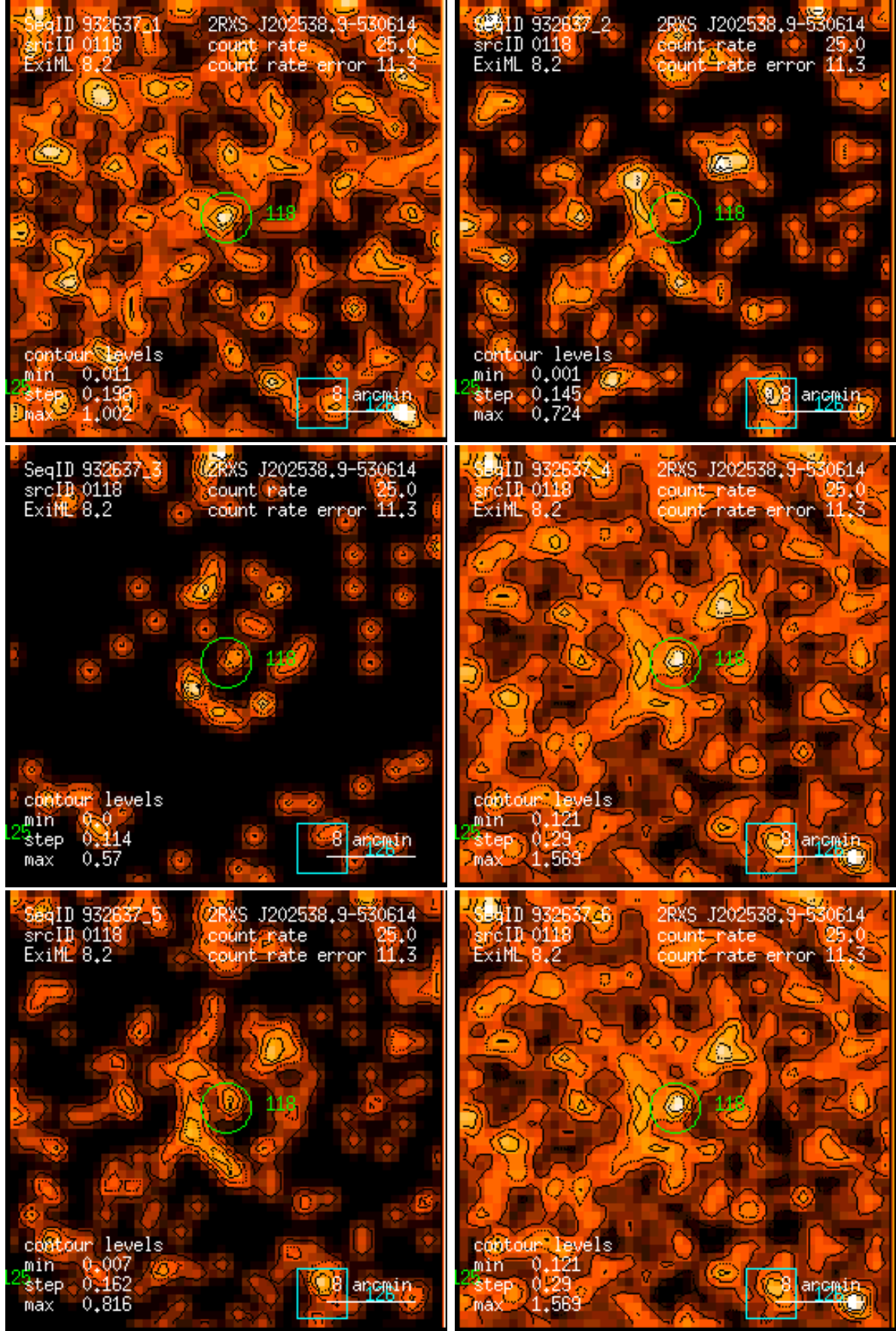
Figure 118: RASS 932637: detection 0118: band rate images, Gaussian filter: (1) PSPC channels 11 – 41, (2) 52 – 90, (3) 91 – 201, (4) 11 – 235, (5) 52 – 201, (6) 11 – 201. Broad band rates in counts/ks. Band rate contour levels in counts/ks/arcmin 2 .
