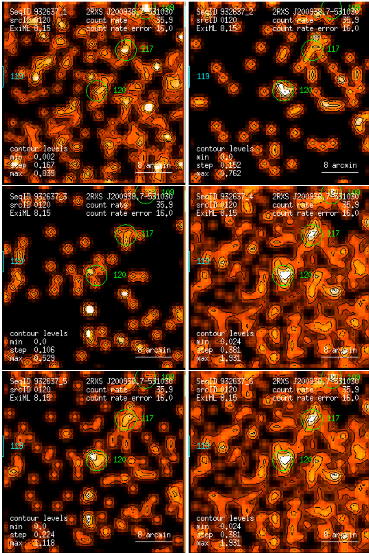
Figure 120: RASS 932637: detection 0120: band rate images, Gaussian filter: (1) PSPC channels 11 – 41, (2) 52 – 90, (3) 91 – 201, (4) 11 – 235, (5) 52 – 201, (6) 11 – 201. Broad band rates in counts/ks. Band rate contour levels in counts/ks/arcmin 2 .
