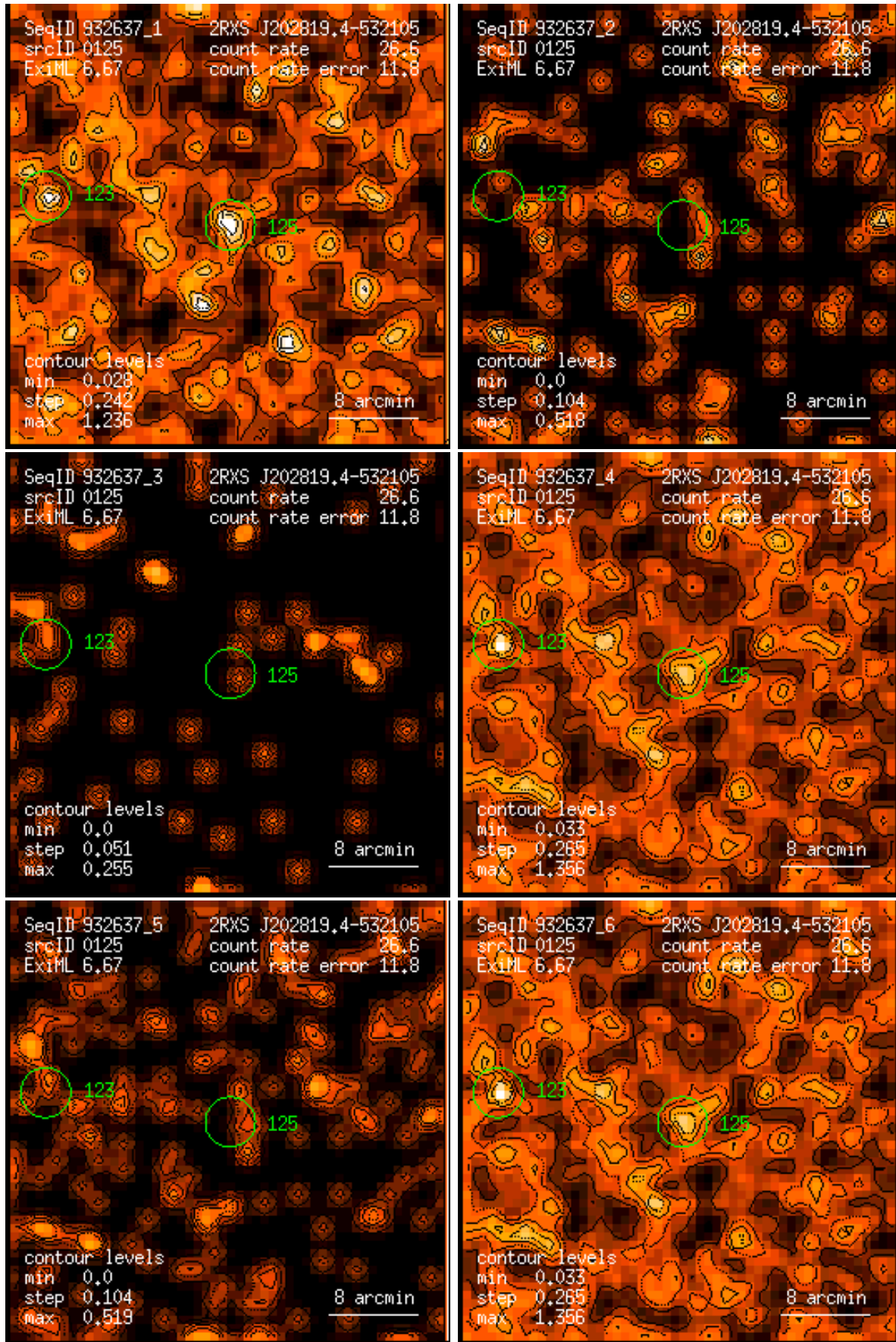
Figure 125: RASS 932637: detection 0125: band rate images, Gaussian filter: (1) PSPC channels 11 – 41, (2) 52 – 90, (3) 91 – 201, (4) 11 – 235, (5) 52 – 201, (6) 11 – 201. Broad band rates in counts/ks. Band rate contour levels in counts/ks/arcmin 2 .
