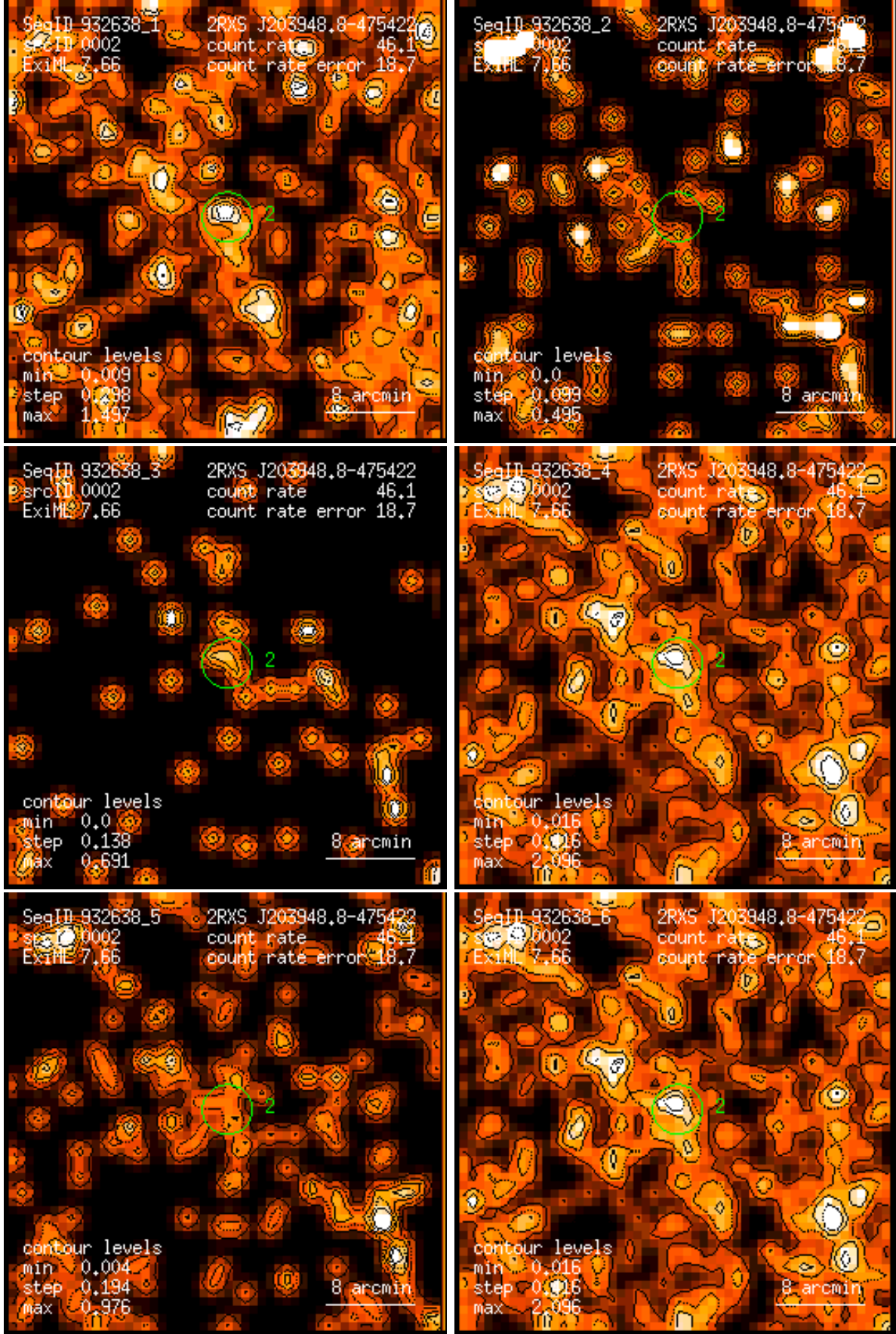
Figure 2: RASS 932638: detection 0002: band rate images, Gaussian filter: (1) PSPC channels 11 – 41, (2) 52 – 90, (3) 91 – 201, (4) 11 – 235, (5) 52 – 201, (6) 11 – 201. Broad band rates in counts/ks. Band rate contour levels in counts/ks/arcmin 2 .
