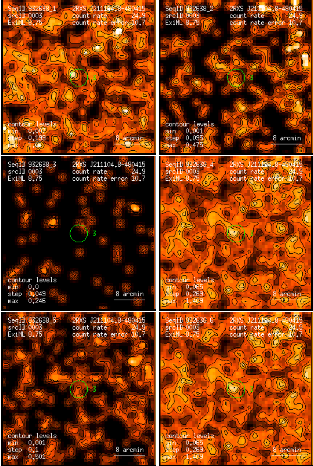
Figure 3: RASS 932638: detection 0003: band rate images, Gaussian filter: (1) PSPC channels 11 – 41, (2) 52 – 90, (3) 91 – 201, (4) 11 – 235, (5) 52 – 201, (6) 11 – 201. Broad band rates in counts/ks. Band rate contour levels in counts/ks/arcmin 2 .
