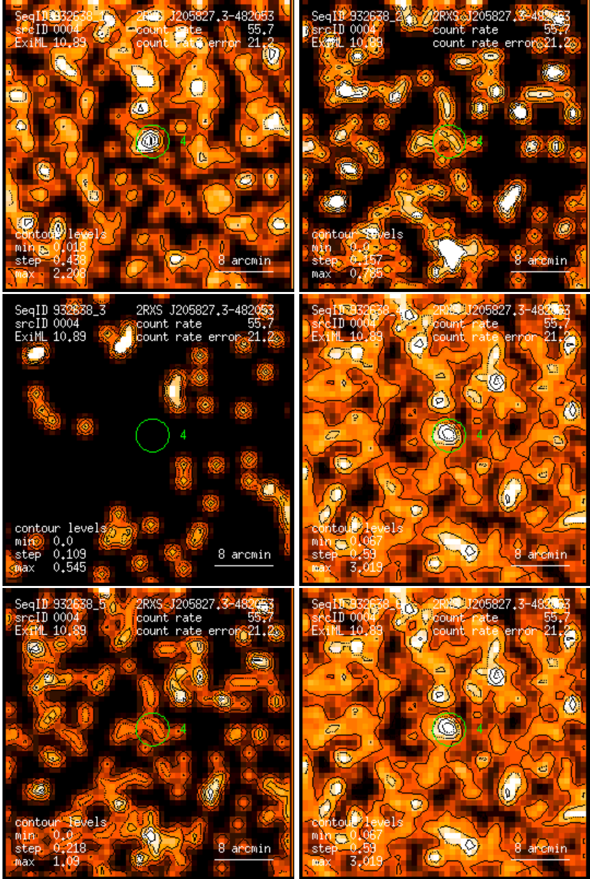
Figure 4: RASS 932638: detection 0004: band rate images, Gaussian filter: (1) PSPC channels 11 – 41, (2) 52 – 90, (3) 91 – 201, (4) 11 – 235, (5) 52 – 201, (6) 11 – 201. Broad band rates in counts/ks. Band rate contour levels in counts/ks/arcmin 2 .
