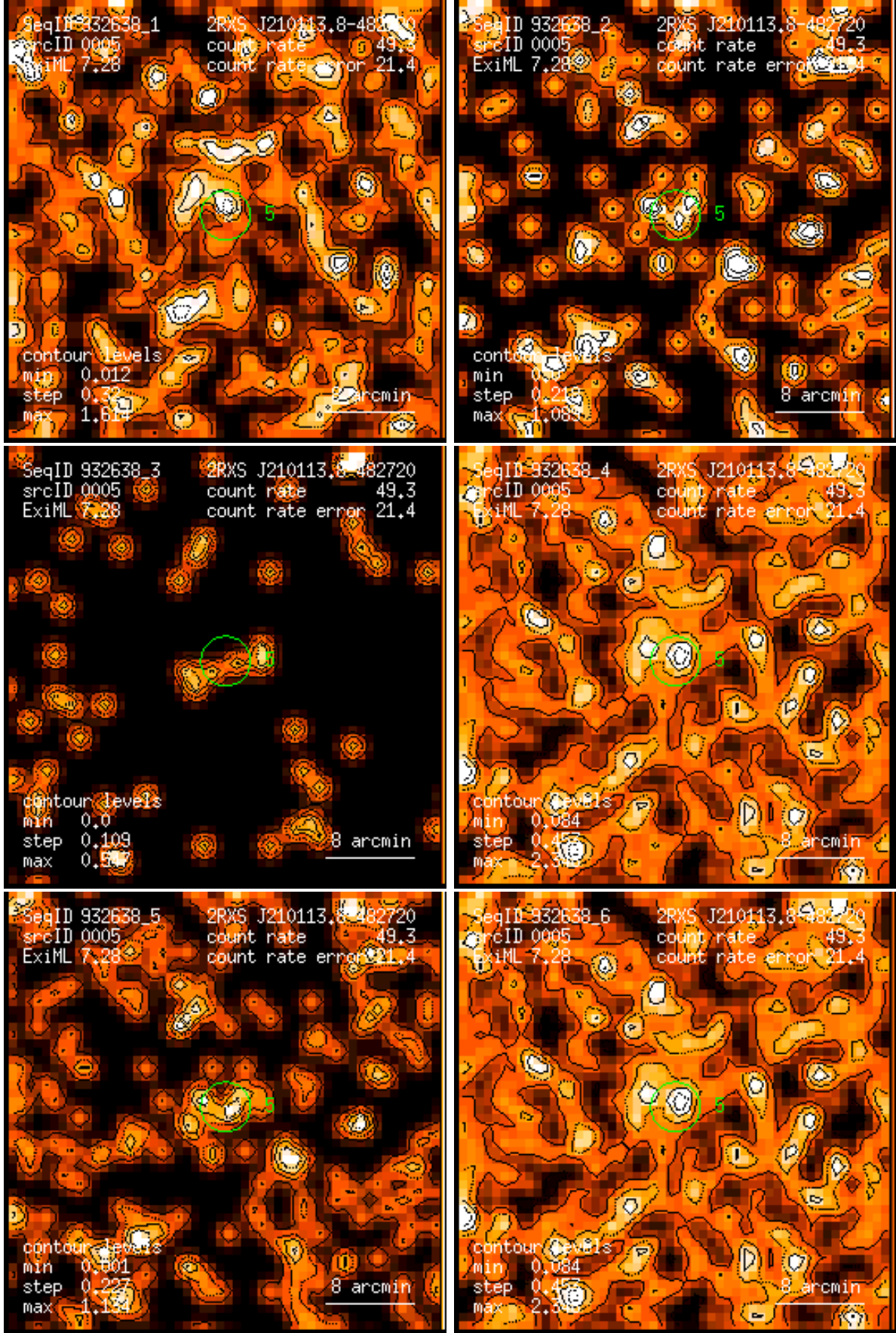
Figure 5: RASS 932638: detection 0005: band rate images, Gaussian filter: (1) PSPC channels 11 – 41, (2) 52 – 90, (3) 91 – 201, (4) 11 – 235, (5) 52 – 201, (6) 11 – 201. Broad band rates in counts/ks. Band rate contour levels in counts/ks/arcmin 2 .
