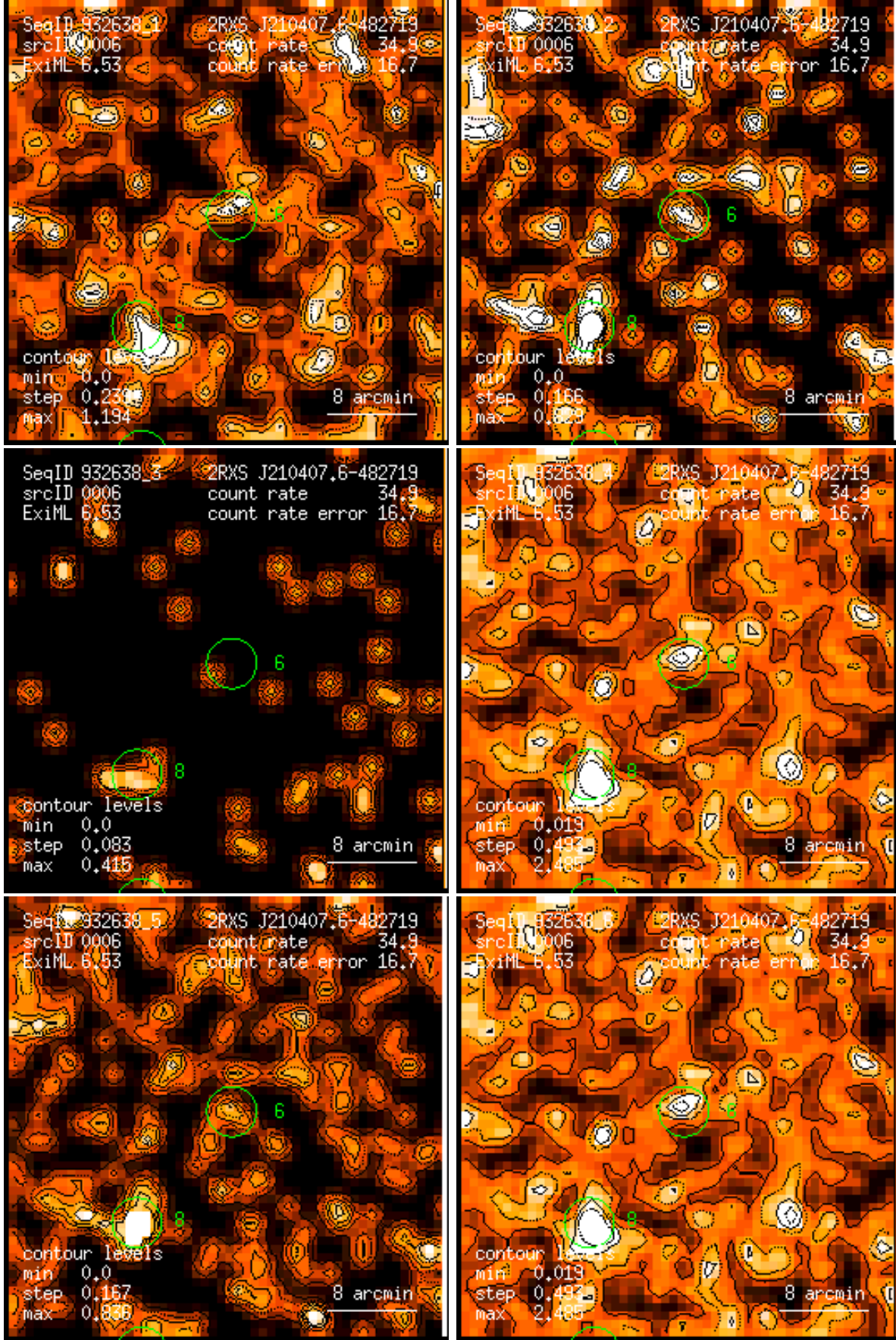
Figure 6: RASS 932638: detection 0006: band rate images, Gaussian filter: (1) PSPC channels 11 – 41, (2) 52 – 90, (3) 91 – 201, (4) 11 – 235, (5) 52 – 201, (6) 11 – 201. Broad band rates in counts/ks. Band rate contour levels in counts/ks/arcmin 2 .
