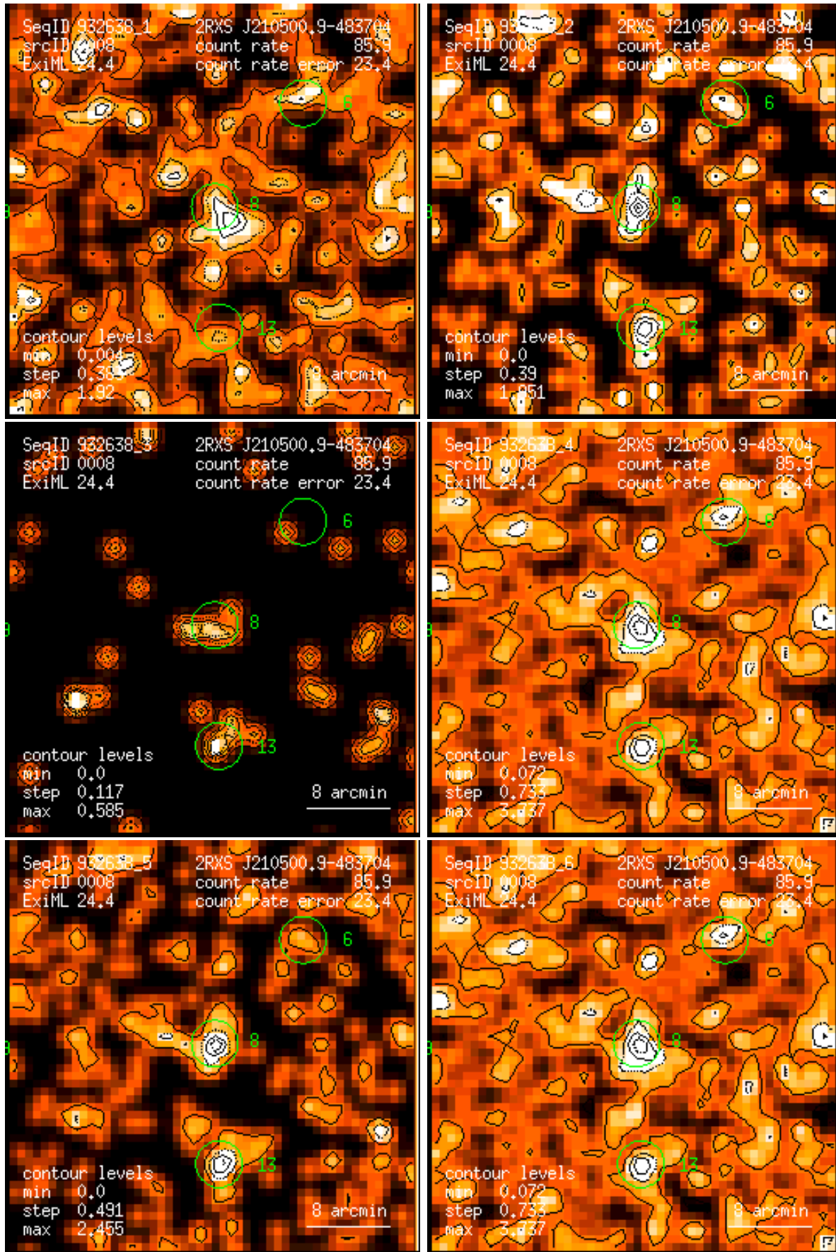
Figure 8: RASS 932638: detection 0008: band rate images, Gaussian filter: (1) PSPC channels 11 – 41, (2) 52 – 90, (3) 91 – 201, (4) 11 – 235, (5) 52 – 201, (6) 11 – 201. Broad band rates in counts/ks. Band rate contour levels in counts/ks/arcmin 2 .
