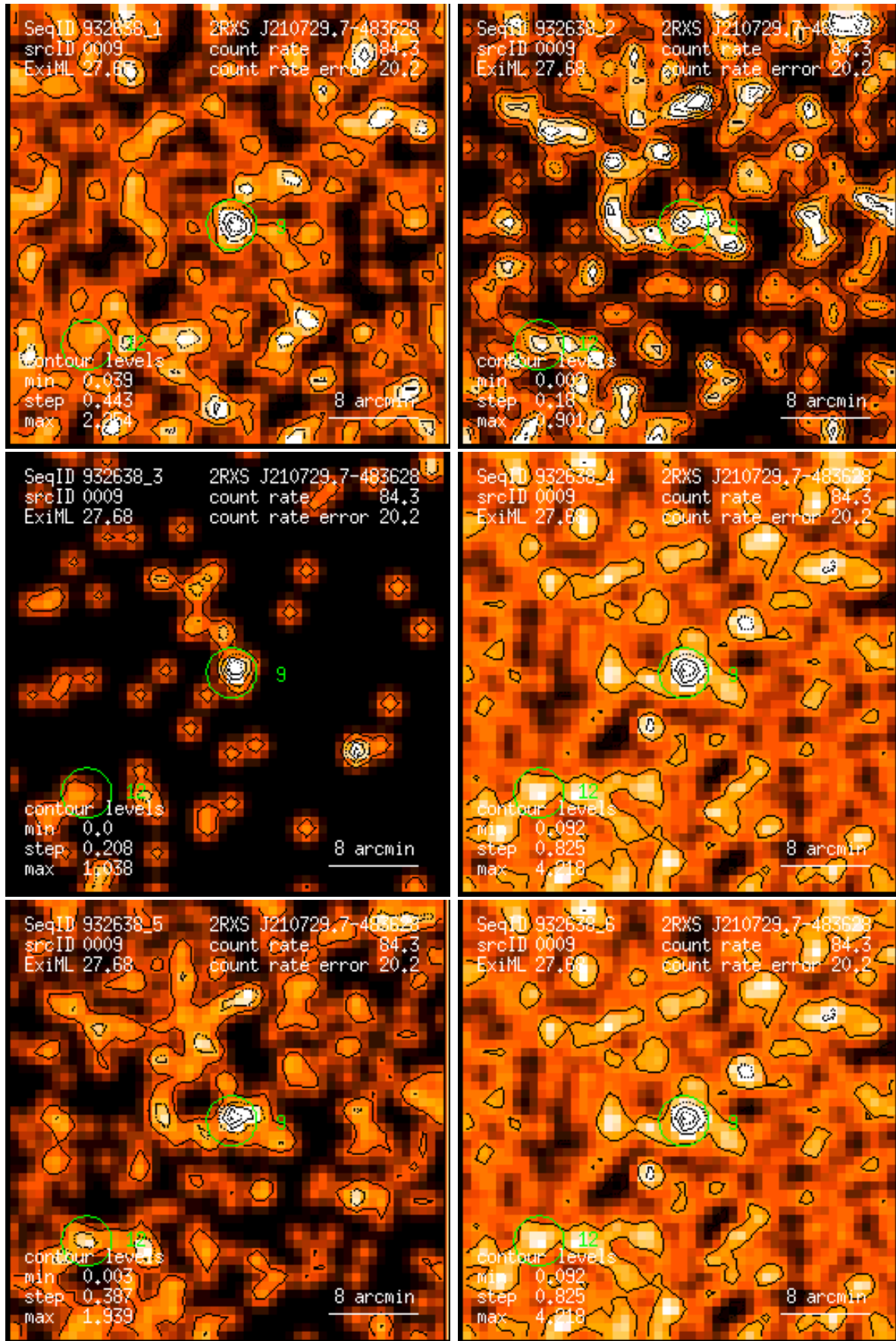
Figure 9: RASS 932638: detection 0009: band rate images, Gaussian filter: (1) PSPC channels 11 – 41, (2) 52 – 90, (3) 91 – 201, (4) 11 – 235, (5) 52 – 201, (6) 11 – 201. Broad band rates in counts/ks. Band rate contour levels in counts/ks/arcmin 2 .
