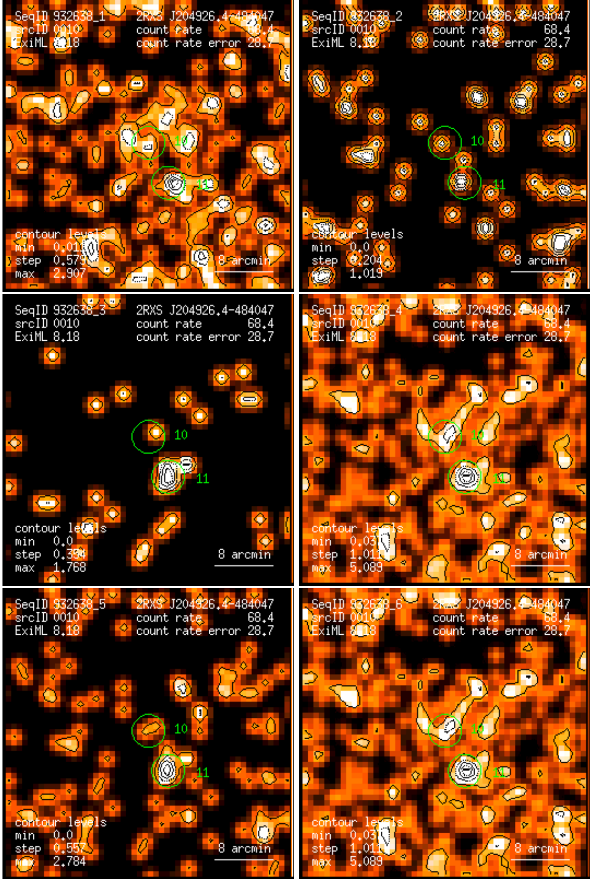
Figure 10: RASS 932638: detection 0010: band rate images, Gaussian filter: (1) PSPC channels 11 – 41, (2) 52 – 90, (3) 91 – 201, (4) 11 – 235, (5) 52 – 201, (6) 11 – 201. Broad band rates in counts/ks. Band rate contour levels in counts/ks/arcmin 2 .
