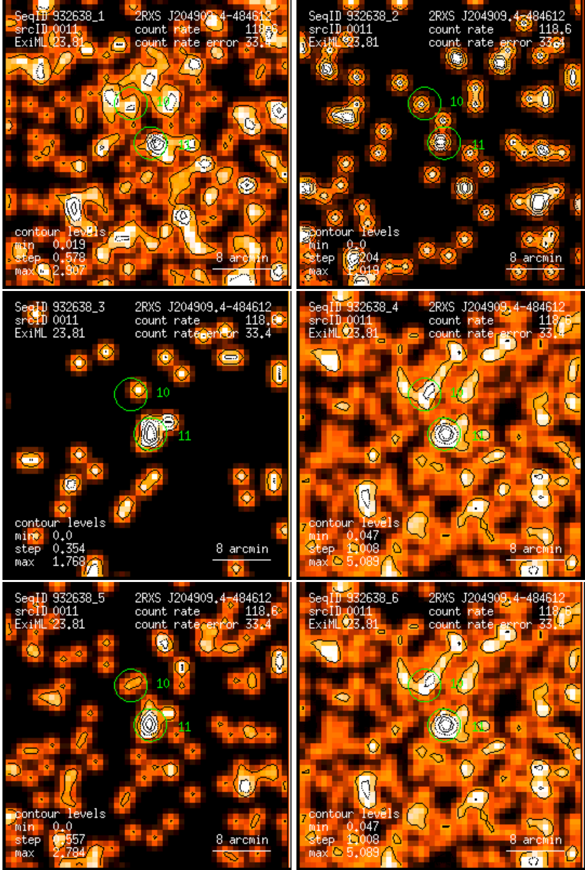
Figure 11: RASS 932638: detection 0011: band rate images, Gaussian filter: (1) PSPC channels 11 – 41, (2) 52 – 90, (3) 91 – 201, (4) 11 – 235, (5) 52 – 201, (6) 11 – 201. Broad band rates in counts/ks. Band rate contour levels in counts/ks/arcmin 2 .
