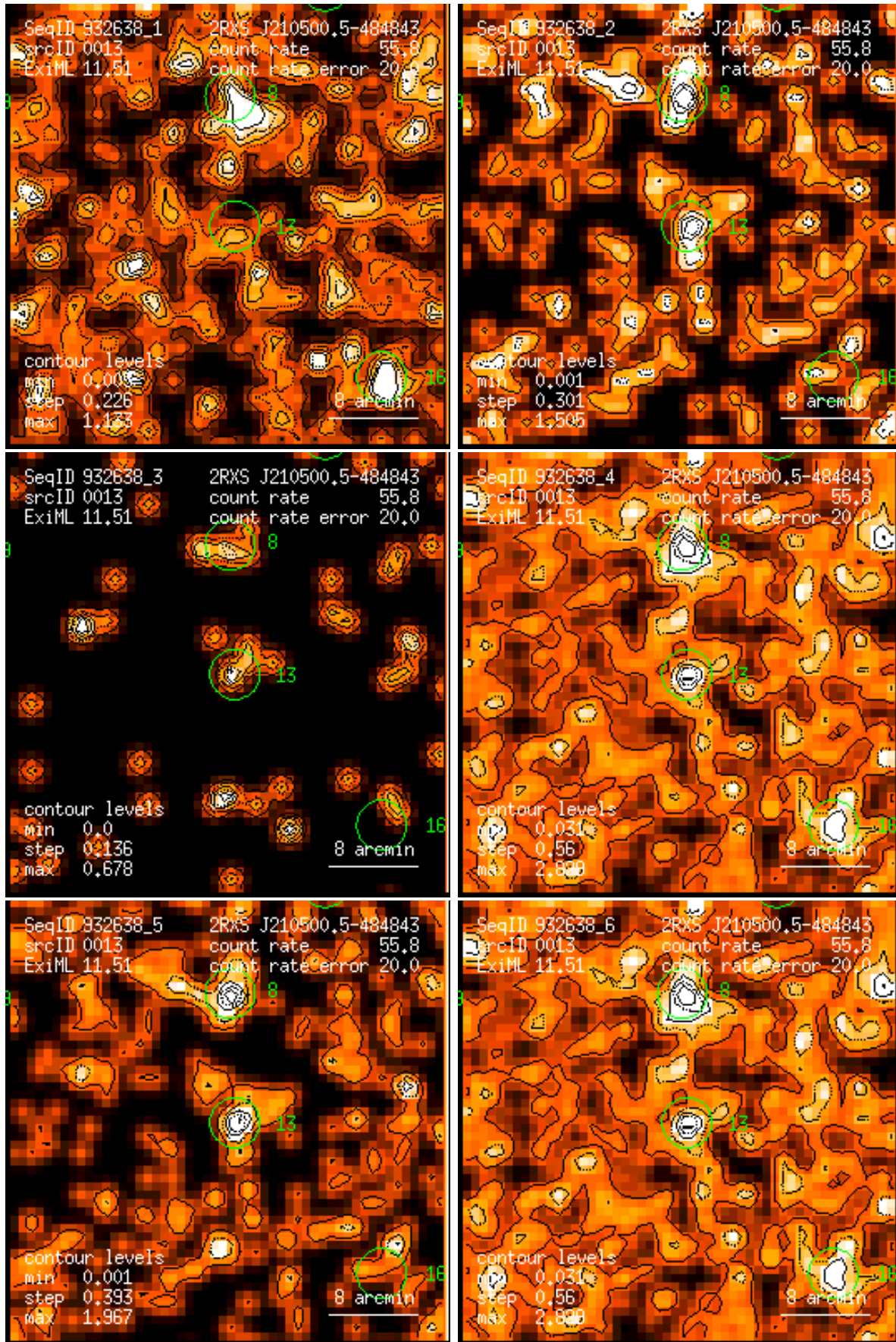
Figure 13: RASS 932638: detection 0013: band rate images, Gaussian filter: (1) PSPC channels 11 – 41, (2) 52 – 90, (3) 91 – 201, (4) 11 – 235, (5) 52 – 201, (6) 11 – 201. Broad band rates in counts/ks. Band rate contour levels in counts/ks/arcmin 2 .
