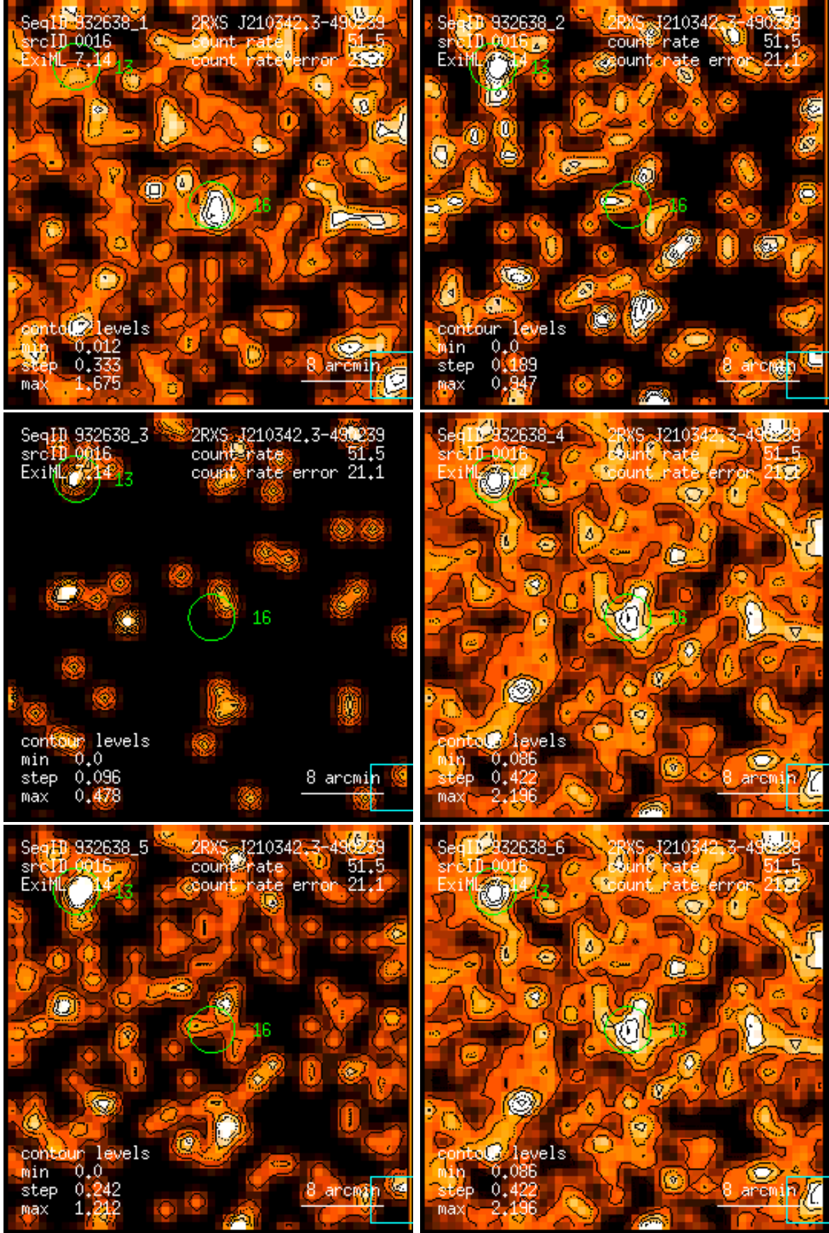
Figure 16: RASS 932638: detection 0016: band rate images, Gaussian filter: (1) PSPC channels 11 – 41, (2) 52 – 90, (3) 91 – 201, (4) 11 – 235, (5) 52 – 201, (6) 11 – 201. Broad band rates in counts/ks. Band rate contour levels in counts/ks/arcmin 2 .
