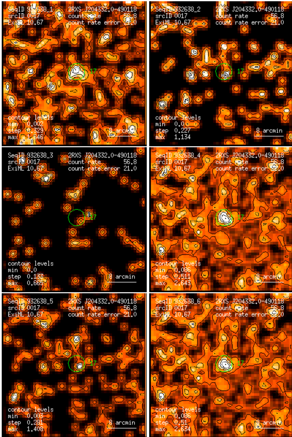
Figure 17: RASS 932638: detection 0017: band rate images, Gaussian filter: (1) PSPC channels 11 – 41, (2) 52 – 90, (3) 91 – 201, (4) 11 – 235, (5) 52 – 201, (6) 11 – 201. Broad band rates in counts/ks. Band rate contour levels in counts/ks/arcmin 2 .
