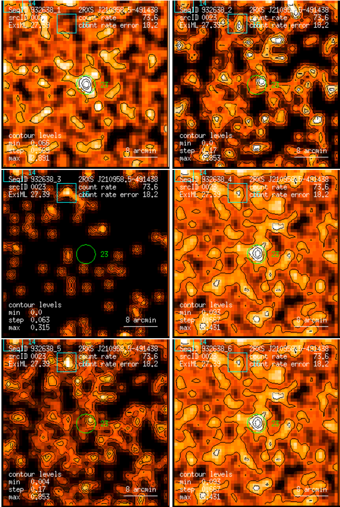
Figure 23: RASS 932638: detection 0023: band rate images, Gaussian filter: (1) PSPC channels 11 – 41, (2) 52 – 90, (3) 91 – 201, (4) 11 – 235, (5) 52 – 201, (6) 11 – 201. Broad band rates in counts/ks. Band rate contour levels in counts/ks/arcmin 2 .
