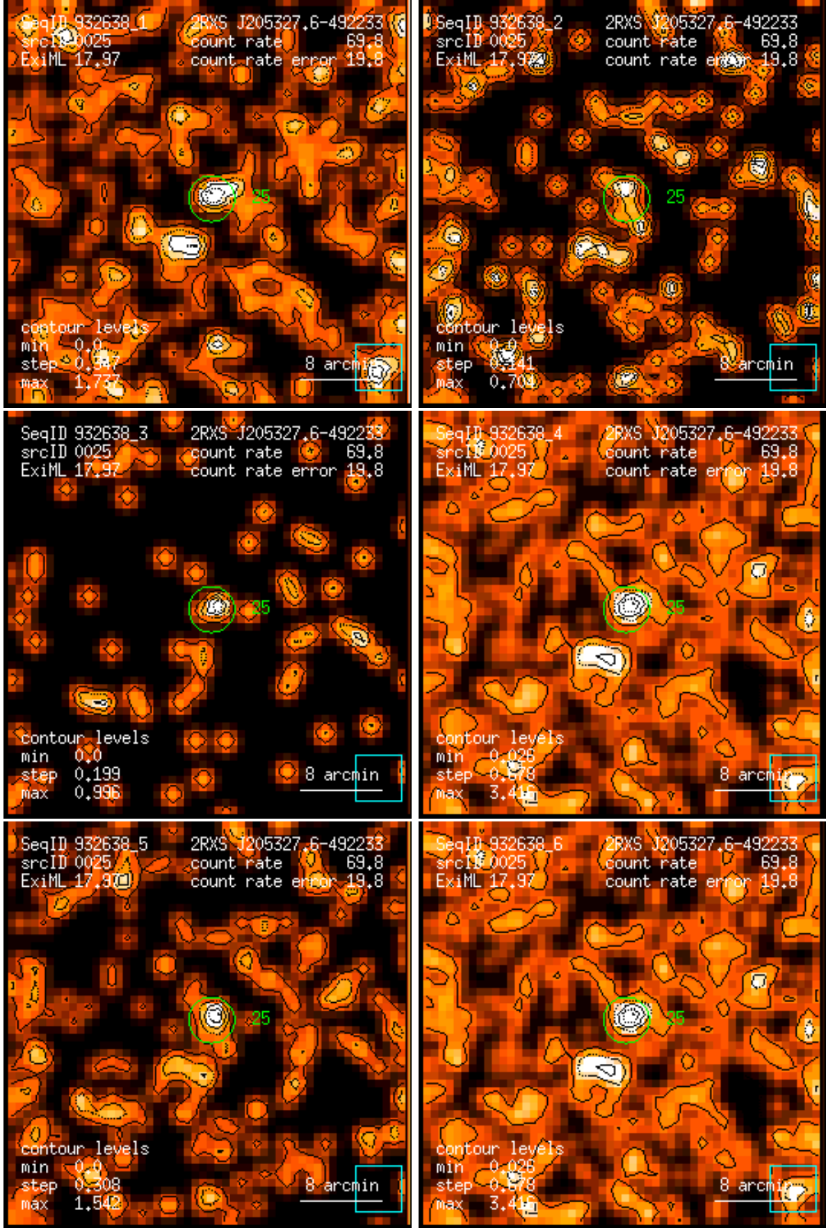
Figure 25: RASS 932638: detection 0025: band rate images, Gaussian filter: (1) PSPC channels 11 – 41, (2) 52 – 90, (3) 91 – 201, (4) 11 – 235, (5) 52 – 201, (6) 11 – 201. Broad band rates in counts/ks. Band rate contour levels in counts/ks/arcmin 2 .
