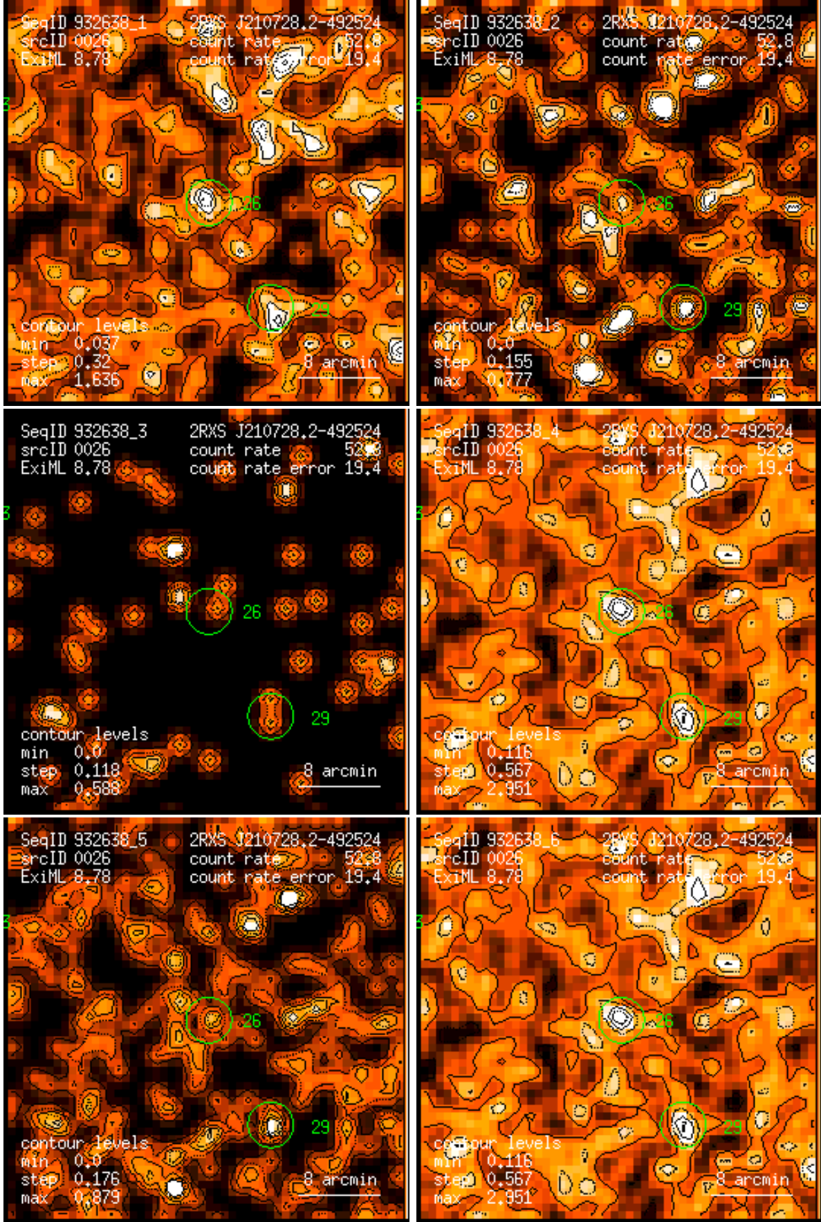
Figure 26: RASS 932638: detection 0026: band rate images, Gaussian filter: (1) PSPC channels 11 – 41, (2) 52 – 90, (3) 91 – 201, (4) 11 – 235, (5) 52 – 201, (6) 11 – 201. Broad band rates in counts/ks. Band rate contour levels in counts/ks/arcmin 2 .
