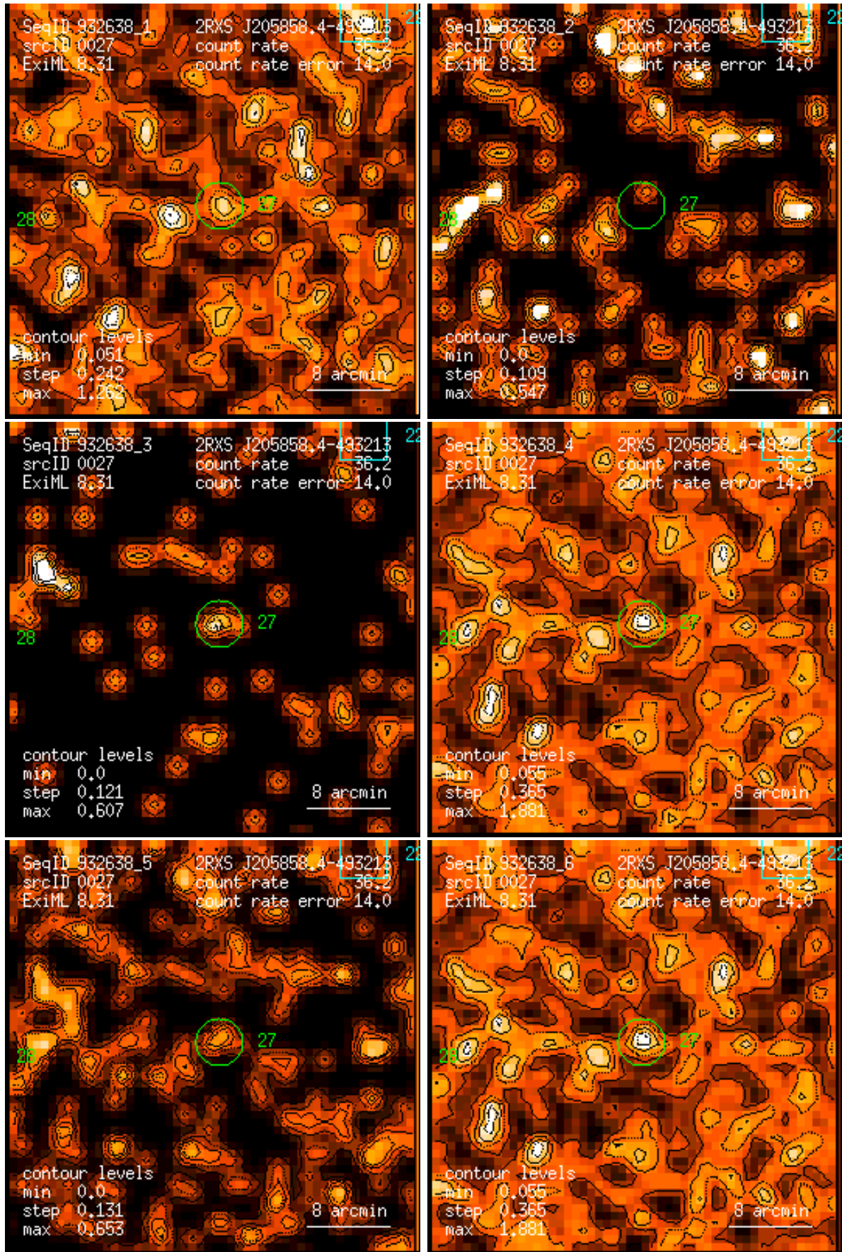
Figure 27: RASS 932638: detection 0027: band rate images, Gaussian filter: (1) PSPC channels 11 – 41, (2) 52 – 90, (3) 91 – 201, (4) 11 – 235, (5) 52 – 201, (6) 11 – 201. Broad band rates in counts/ks. Band rate contour levels in counts/ks/arcmin 2 .
