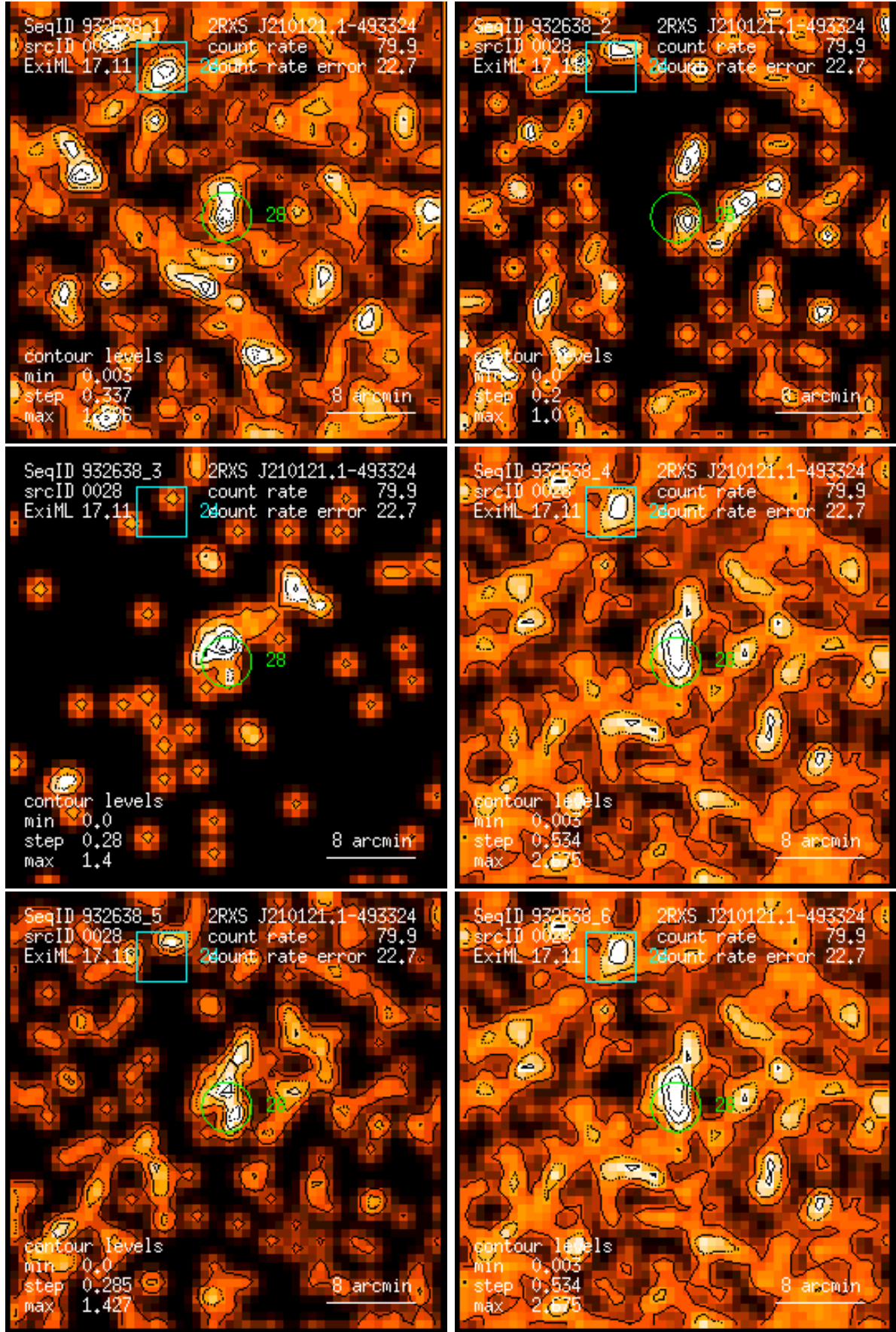
Figure 28: RASS 932638: detection 0028: band rate images, Gaussian filter: (1) PSPC channels 11 – 41, (2) 52 – 90, (3) 91 – 201, (4) 11 – 235, (5) 52 – 201, (6) 11 – 201. Broad band rates in counts/ks. Band rate contour levels in counts/ks/arcmin 2 .
