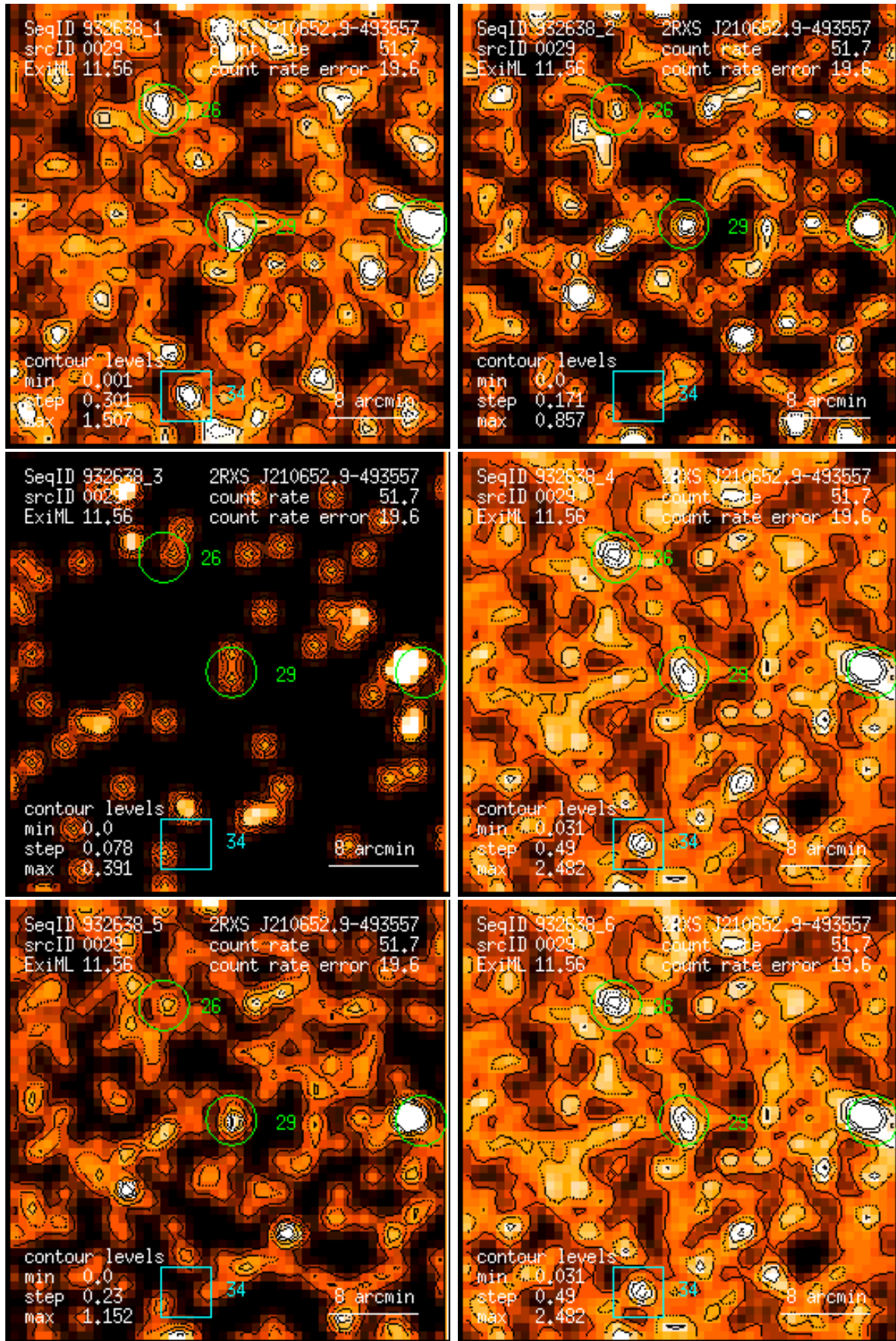
Figure 29: RASS 932638: detection 0029: band rate images, Gaussian filter: (1) PSPC channels 11 – 41, (2) 52 – 90, (3) 91 – 201, (4) 11 – 235, (5) 52 – 201, (6) 11 – 201. Broad band rates in counts/ks. Band rate contour levels in counts/ks/arcmin 2 .
