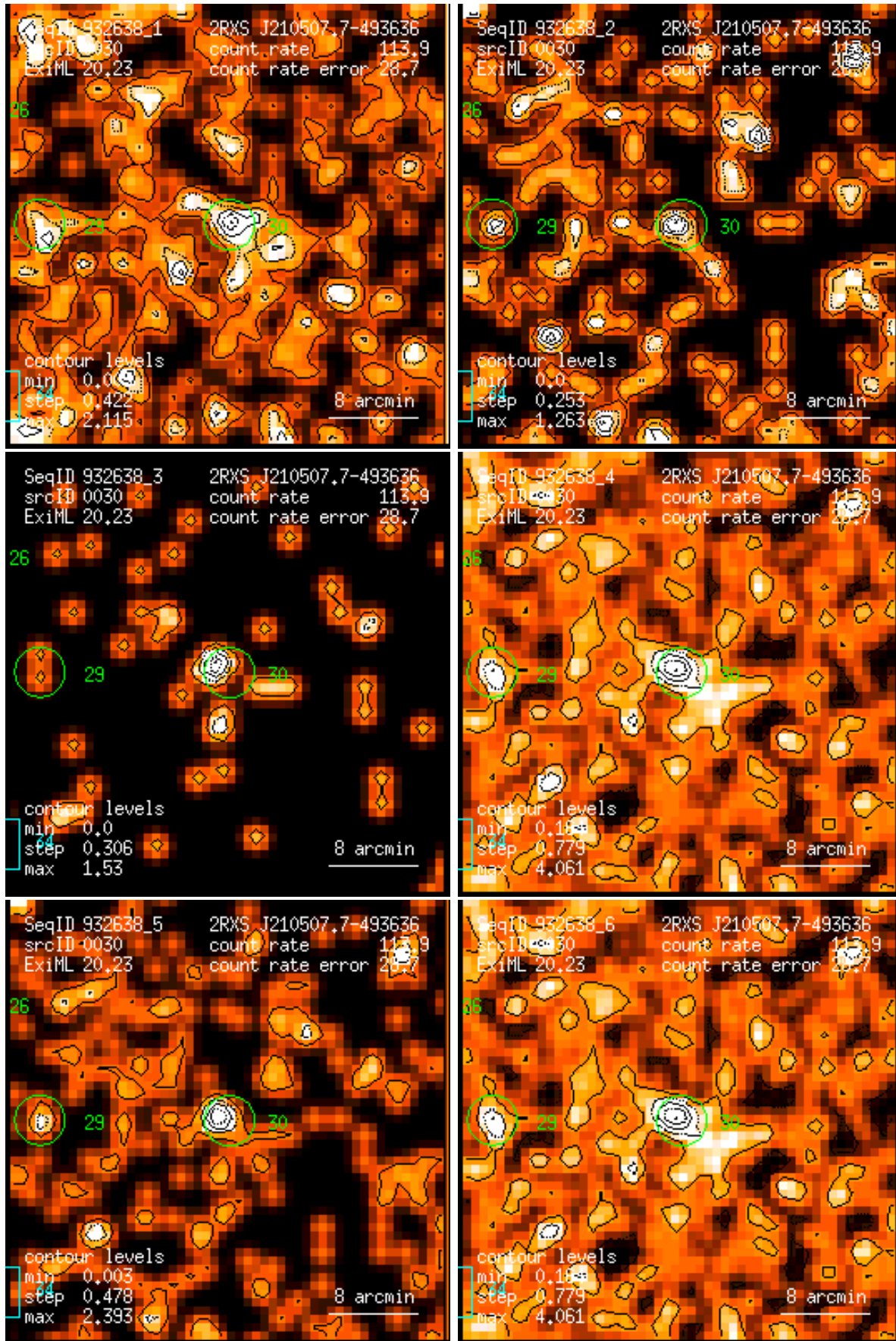
Figure 30: RASS 932638: detection 0030: band rate images, Gaussian filter: (1) PSPC channels 11 – 41, (2) 52 – 90, (3) 91 – 201, (4) 11 – 235, (5) 52 – 201, (6) 11 – 201. Broad band rates in counts/ks. Band rate contour levels in counts/ks/arcmin 2 .
