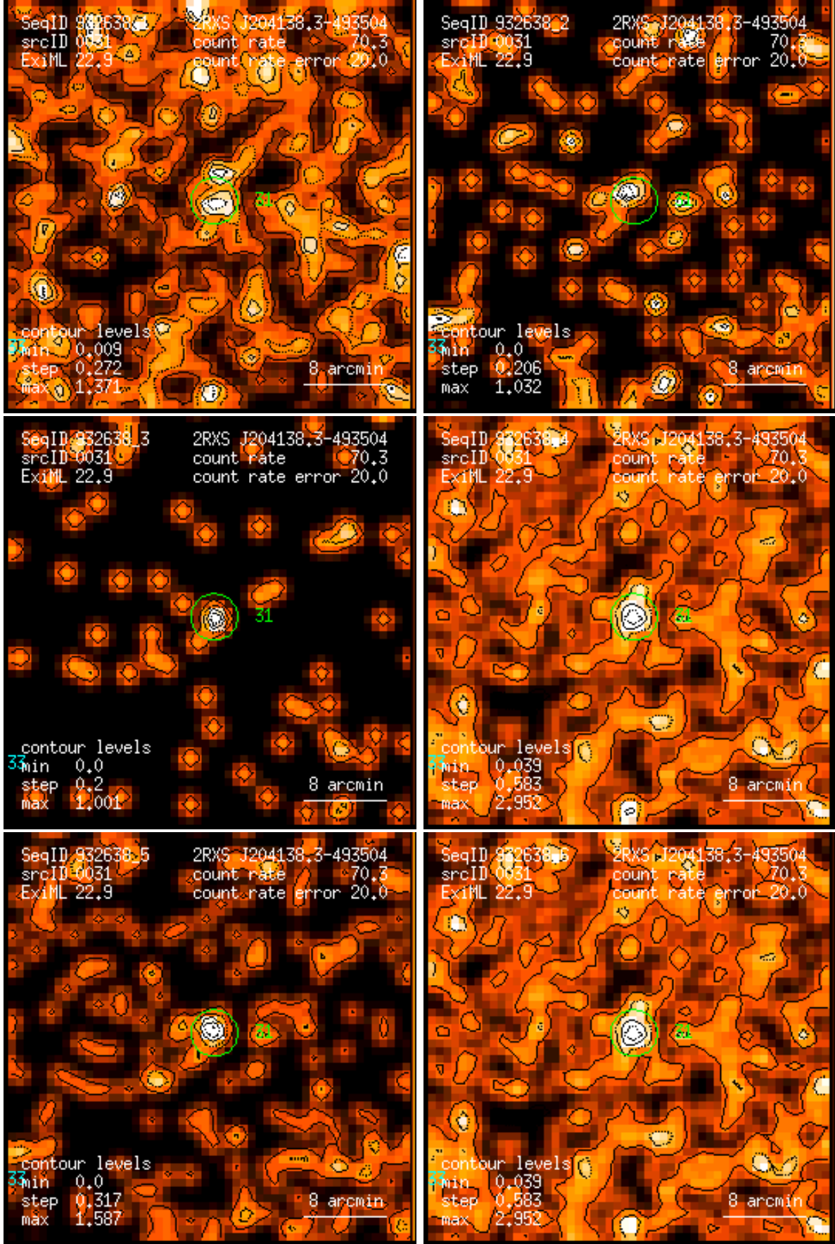
Figure 31: RASS 932638: detection 0031: band rate images, Gaussian filter: (1) PSPC channels 11 – 41, (2) 52 – 90, (3) 91 – 201, (4) 11 – 235, (5) 52 – 201, (6) 11 – 201. Broad band rates in counts/ks. Band rate contour levels in counts/ks/arcmin 2 .
