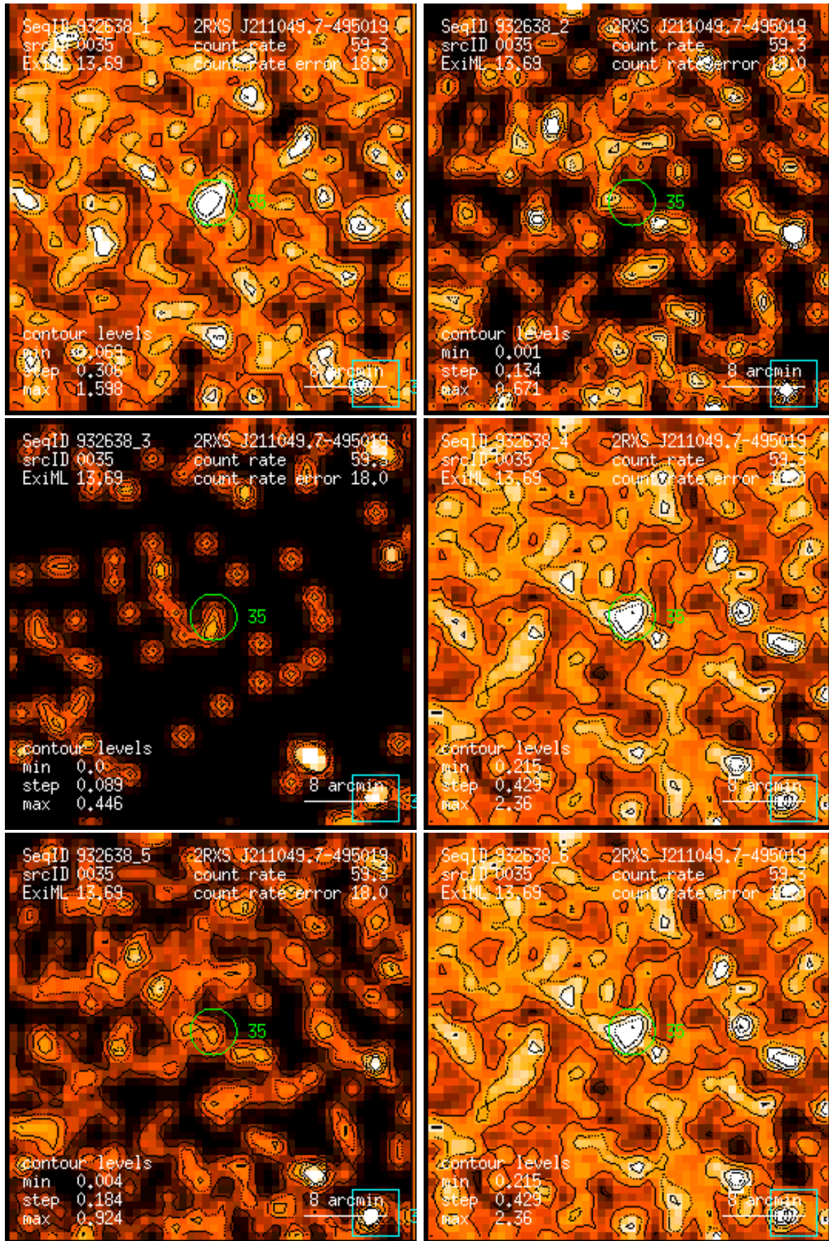
Figure 35: RASS 932638: detection 0035: band rate images, Gaussian filter: (1) PSPC channels 11 – 41, (2) 52 – 90, (3) 91 – 201, (4) 11 – 235, (5) 52 – 201, (6) 11 – 201. Broad band rates in counts/ks. Band rate contour levels in counts/ks/arcmin 2 .
