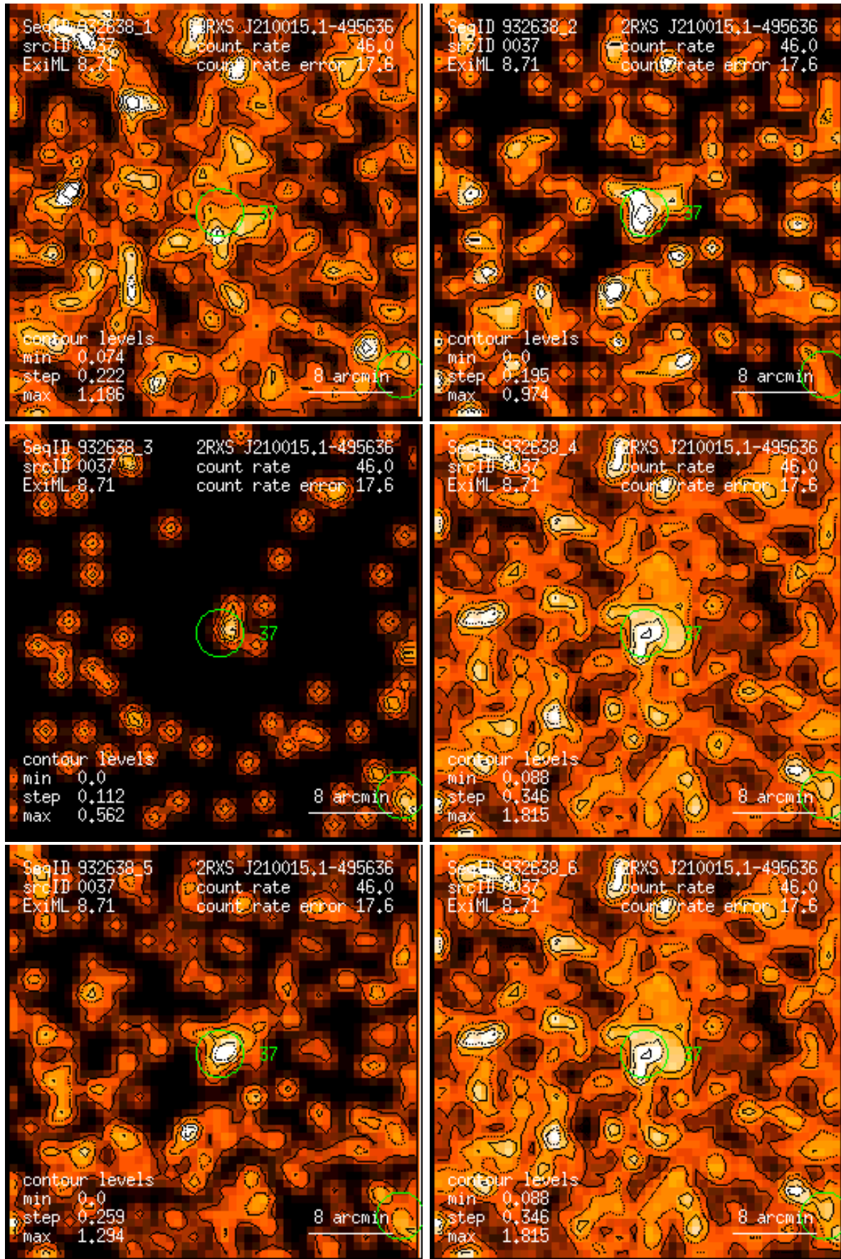
Figure 37: RASS 932638: detection 0037: band rate images, Gaussian filter: (1) PSPC channels 11 – 41, (2) 52 – 90, (3) 91 – 201, (4) 11 – 235, (5) 52 – 201, (6) 11 – 201. Broad band rates in counts/ks. Band rate contour levels in counts/ks/arcmin 2 .
