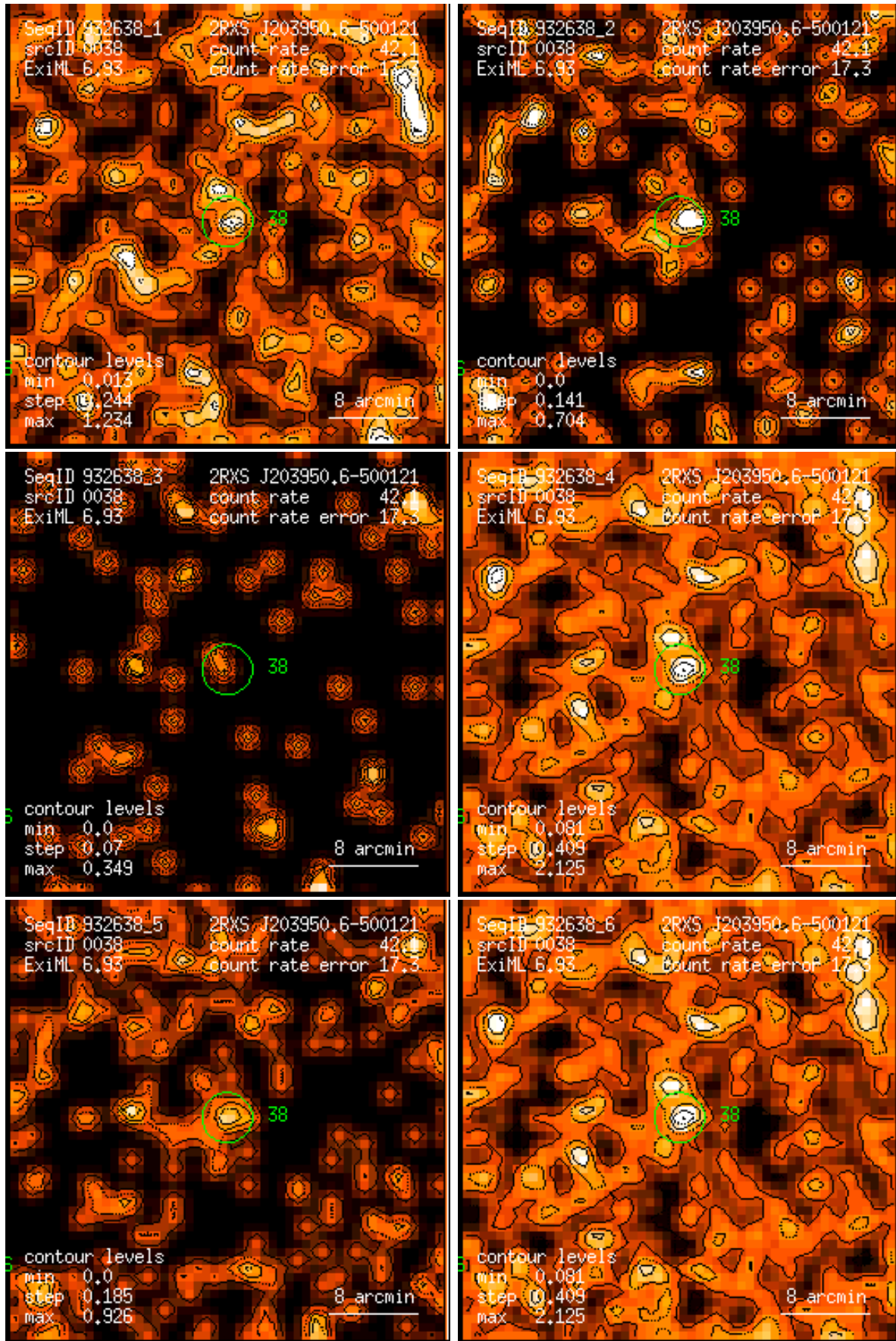
Figure 38: RASS 932638: detection 0038: band rate images, Gaussian filter: (1) PSPC channels 11 – 41, (2) 52 – 90, (3) 91 – 201, (4) 11 – 235, (5) 52 – 201, (6) 11 – 201. Broad band rates in counts/ks. Band rate contour levels in counts/ks/arcmin 2 .
