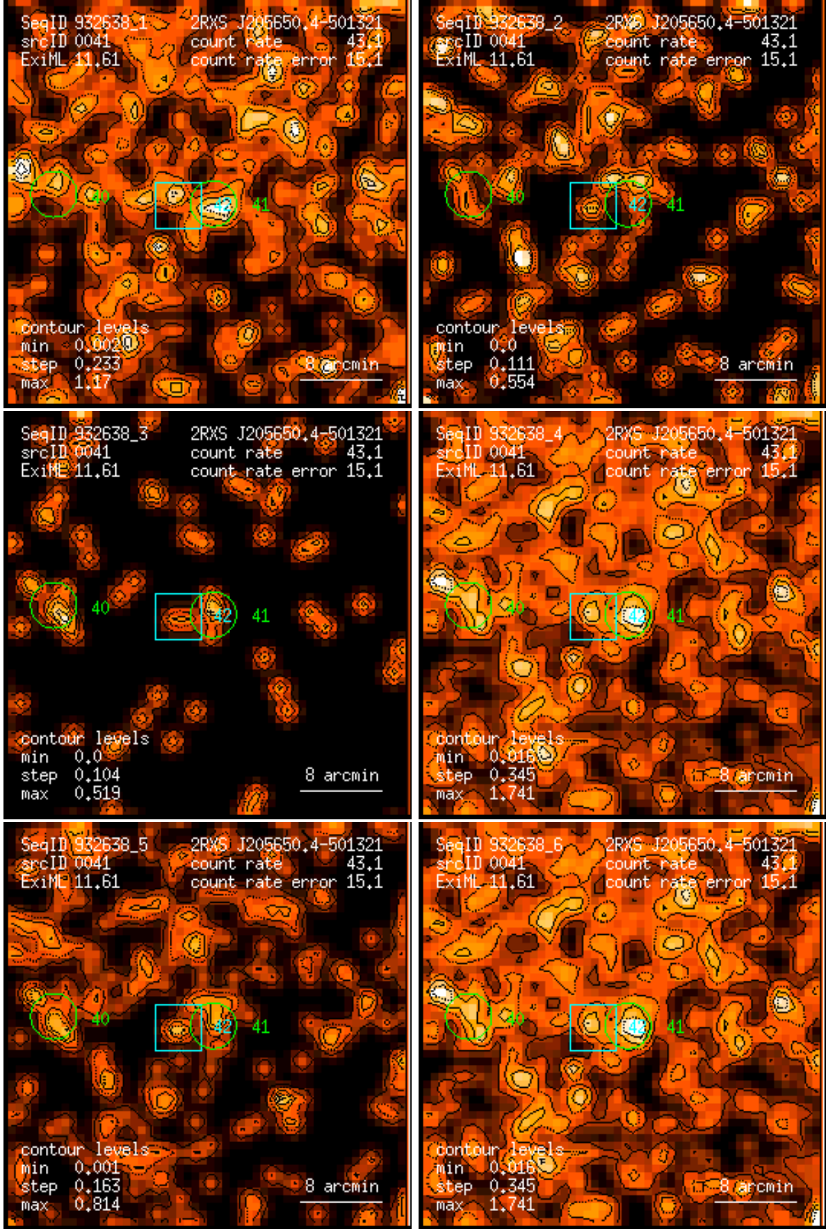
Figure 41: RASS 932638: detection 0041: band rate images, Gaussian filter: (1) PSPC channels 11 – 41, (2) 52 – 90, (3) 91 – 201, (4) 11 – 235, (5) 52 – 201, (6) 11 – 201. Broad band rates in counts/ks. Band rate contour levels in counts/ks/arcmin 2 .
