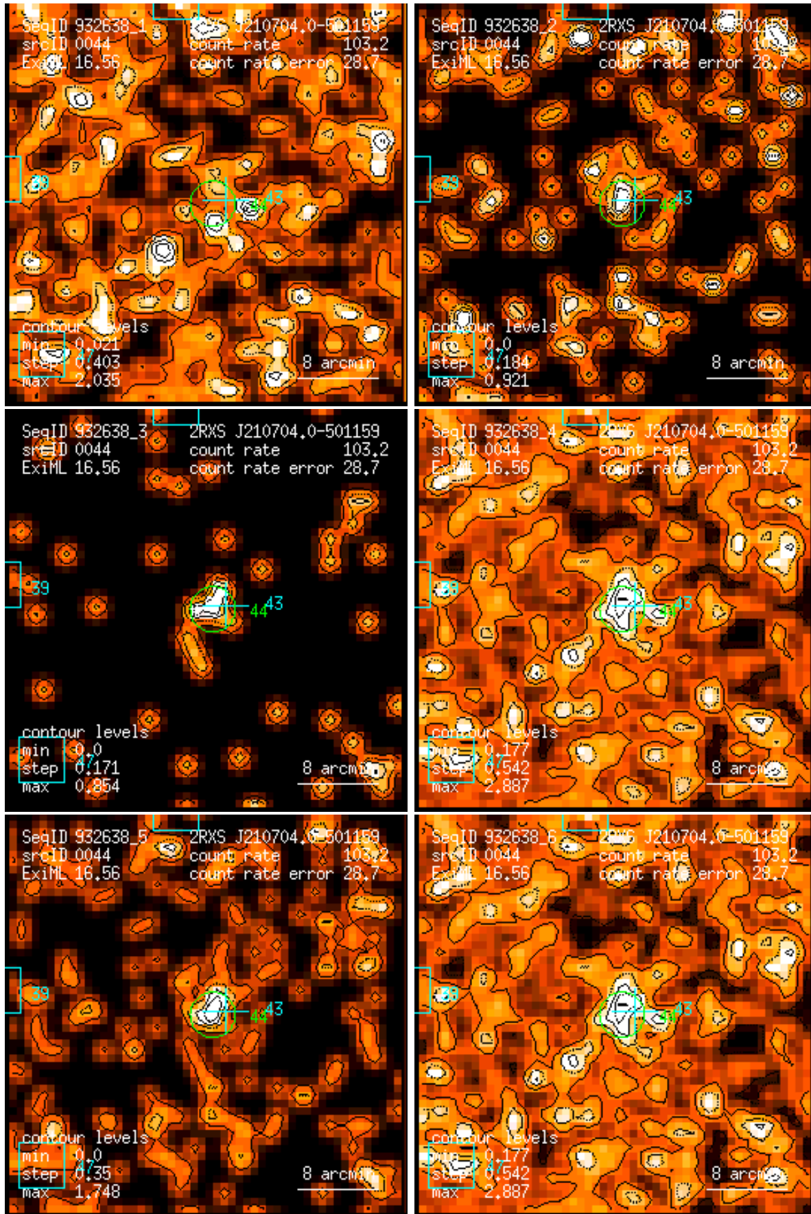
Figure 44: RASS 932638: detection 0044: band rate images, Gaussian filter: (1) PSPC channels 11 – 41, (2) 52 – 90, (3) 91 – 201, (4) 11 – 235, (5) 52 – 201, (6) 11 – 201. Broad band rates in counts/ks. Band rate contour levels in counts/ks/arcmin 2 .
