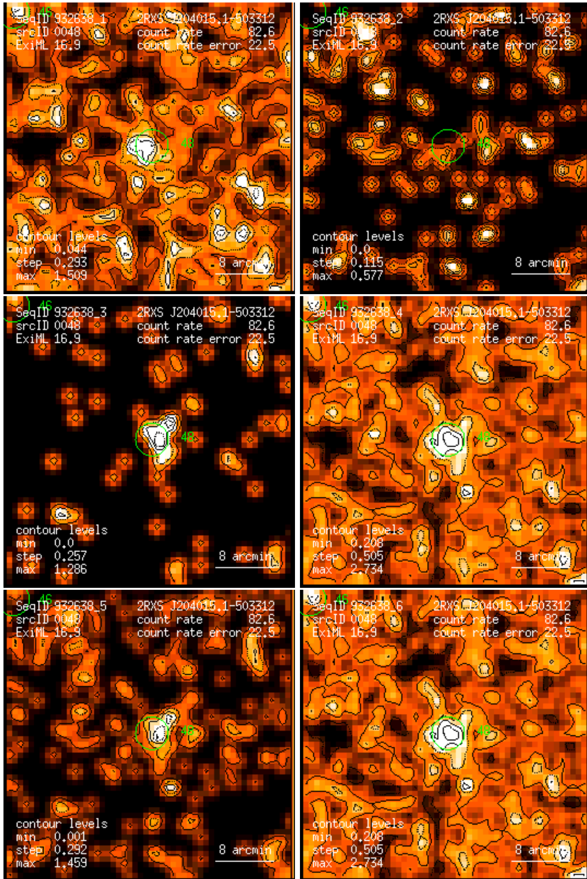
Figure 48: RASS 932638: detection 0048: band rate images, Gaussian filter: (1) PSPC channels 11 – 41, (2) 52 – 90, (3) 91 – 201, (4) 11 – 235, (5) 52 – 201, (6) 11 – 201. Broad band rates in counts/ks. Band rate contour levels in counts/ks/arcmin 2 .
