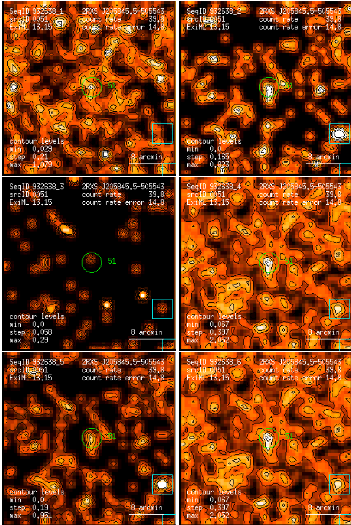
Figure 51: RASS 932638: detection 0051: band rate images, Gaussian filter: (1) PSPC channels 11 – 41, (2) 52 – 90, (3) 91 – 201, (4) 11 – 235, (5) 52 – 201, (6) 11 – 201. Broad band rates in counts/ks. Band rate contour levels in counts/ks/arcmin 2 .
