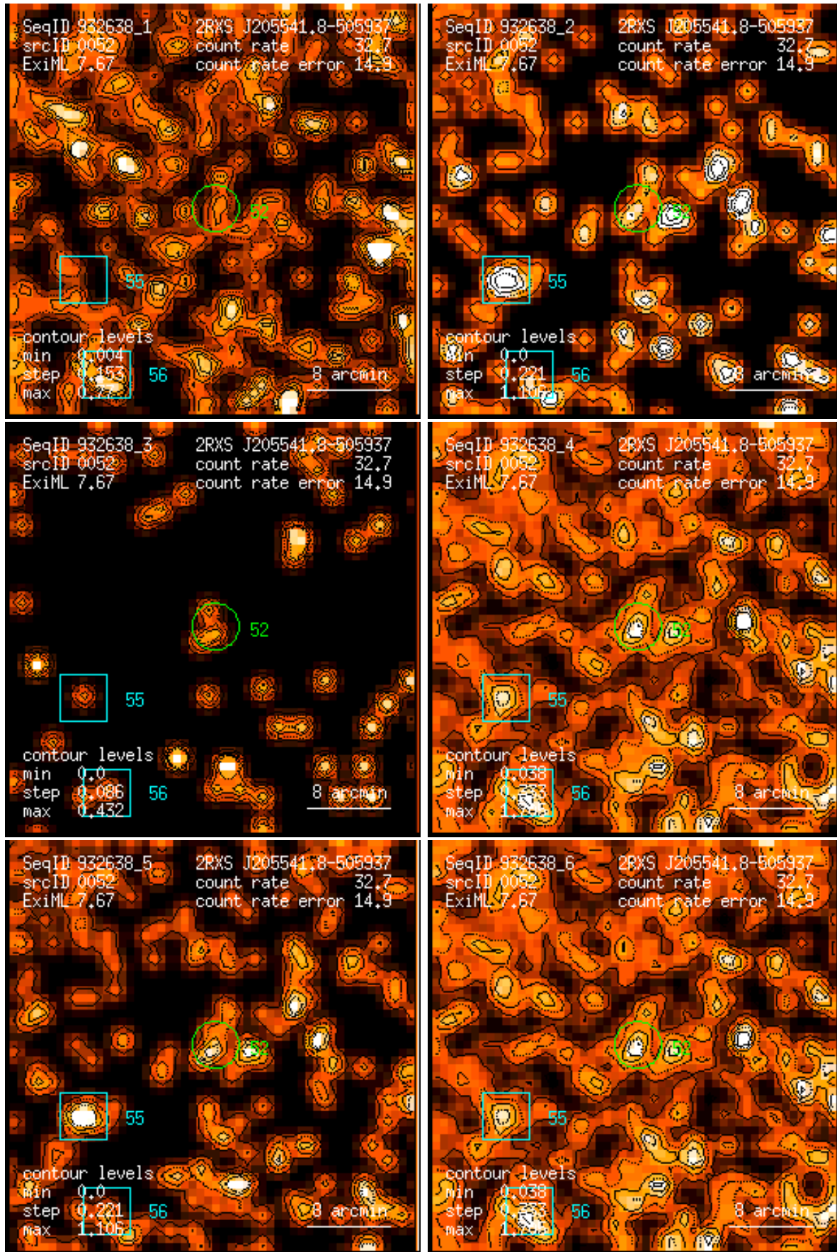
Figure 52: RASS 932638: detection 0052: band rate images, Gaussian filter: (1) PSPC channels 11 – 41, (2) 52 – 90, (3) 91 – 201, (4) 11 – 235, (5) 52 – 201, (6) 11 – 201. Broad band rates in counts/ks. Band rate contour levels in counts/ks/arcmin 2 .
