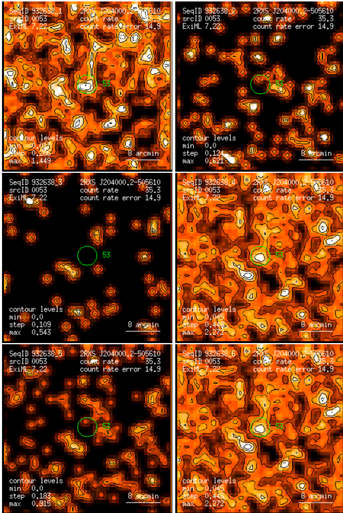
Figure 53: RASS 932638: detection 0053: band rate images, Gaussian filter: (1) PSPC channels 11 – 41, (2) 52 – 90, (3) 91 – 201, (4) 11 – 235, (5) 52 – 201, (6) 11 – 201. Broad band rates in counts/ks. Band rate contour levels in counts/ks/arcmin 2 .
