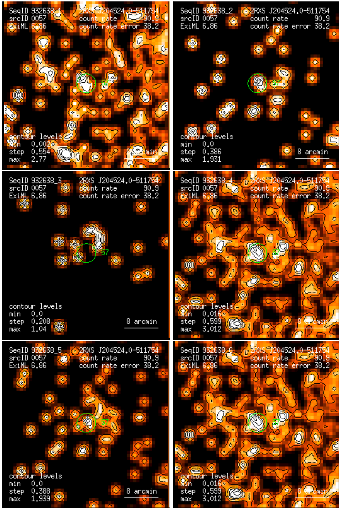
Figure 57: RASS 932638: detection 0057: band rate images, Gaussian filter: (1) PSPC channels 11 – 41, (2) 52 – 90, (3) 91 – 201, (4) 11 – 235, (5) 52 – 201, (6) 11 – 201. Broad band rates in counts/ks. Band rate contour levels in counts/ks/arcmin 2 .
